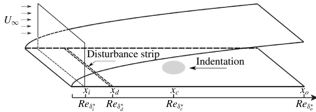
FIGURE 1. Overview of the 3-D computational set-up with the Blasius profile at the inflow and positions of the disturbance strip (double dashed lines) and indentation (grey shading area). x_c denotes the streamwise centre position of indentation. (The parameter definitions can be found in tables 1 and 2.)
