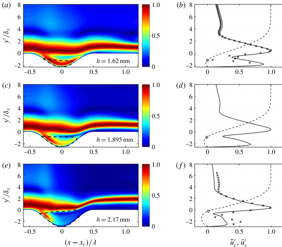
FIGURE 9. (Colour online) Comparisons of |\tilde{u}'(x', y', z')|/A'(x', z') contours (a,c,e) in the planes z' = 0 and corresponding TS mode profiles |\tilde{u}'_c| = |\tilde{u}'(x', y', z')|/A'(x', z') and |\tilde{v}'_c| = |\tilde{v}'(x', y', z')|/A'(x', z') (b,d,f) at x' = x'_c in the planes z' = 0 . The parameter \lambda = 81 mm. (a,b) h = 1.620 mm; (c,d) h = 1.895 mm; (e,f) h = 2.170 mm. In (a,c,e), the dashed lines indicate the interfaces of the regions enclosed by \Gamma = \{(x', y') : \tilde{u}'(x', y', z' = 0) = 0\} and in (b,d,f), the solid lines indicate the profiles of |\tilde{u}'_c| and the dashed lines indicate the profiles of |\tilde{v}'_c| . In (b,d,f), \times symbols indicate the experimental results of |\tilde{u}'_c| and \circ indicates the position where \tilde{u}'_c = 0 .
