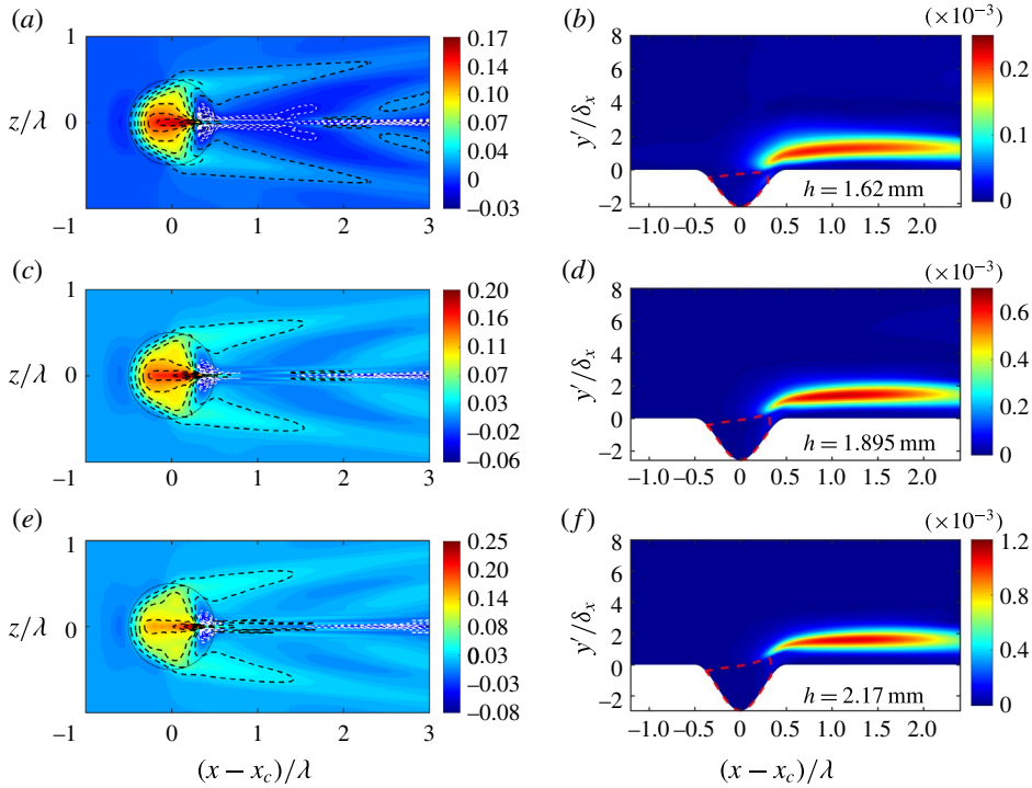
FIGURE 8. (Colour online) Comparisons of streamwise growth rate \alpha'_\varepsilon contours (a,c,e) and rescaled TS amplitude |\bar{u}'(x', y', z')|/A'(x'_{neutral}, z') contours (b,d,f) where A'(x'_{neutral}, z') means amplitude of TS waves at the lower branch of the neutral stability curve. The parameter \lambda = 40.5 mm. (a,b) h = 1.620 mm; (c,d) h = 1.895 mm; (e,f) h = 2.170 mm. In (a,c,e), the black dashed lines indicate destabilisation of TS waves and the white dashed lines indicate stabilisation of TS waves ( -\alpha'_i \leq 0 ). The solid circles are the curves of r = \lambda/2 . In (b,d,f), the red dashed lines indicate the interfaces of the regions enclosed by \Gamma = \{(x', y') : \bar{u}'(x', y', z' = 0) = 0\} .
