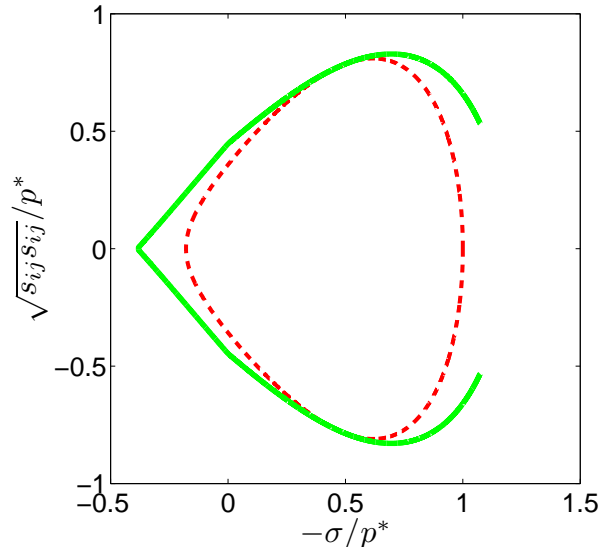
Fig. 5 Sections in the (-\sigma/p^*), (\sqrt{s_{ij}s_{ij}}/p^*) plane through two yield surfaces: a cone at low pressure and a cap at higher pressure, with inter-particle bonding. The solid line shows the yield surface presented in Eq. 35 while the broken line shows that presented in Eq. 28. (See Table 2 for parameter values: c = 0.5 ; \nu_r = 0 ; d_{ii}^g = 0 .)
