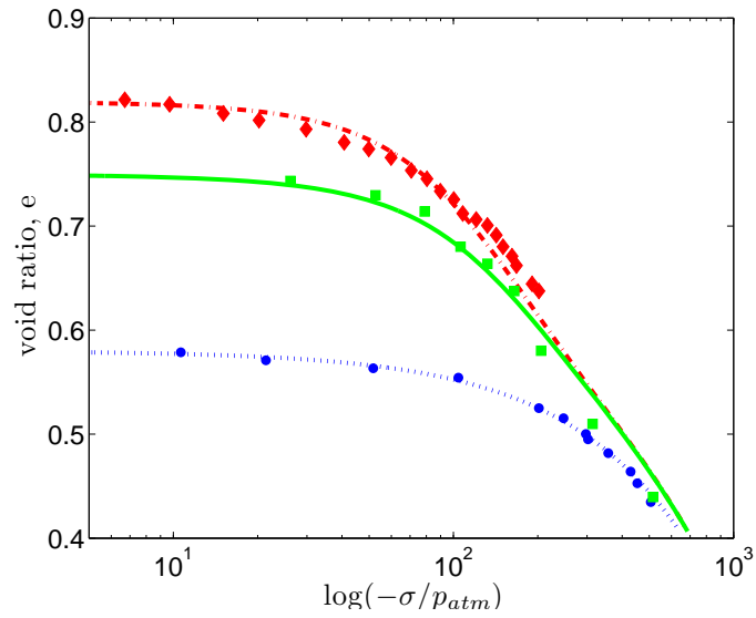
Fig. 10 Simulations (lines) of experiments carried out by Miura (1979); Miura et al (1984) (and represented by Pestana et al (2002b)) on soils with different initial packing densities (diamonds (loose), squares (medium dense) and circles (dense) - redrawn). See Table 3 for parameter values.
