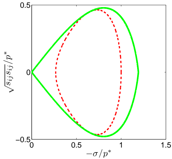
Fig. 4 Sections in the (-\sigma/p^*, (\sqrt{s_{ij}s_{ij}}/p^*)) plane through two yield surfaces: a cone at low pressure and a cap at higher pressure, with no inter-particle bonding. The solid line shows the yield surface presented in Eq. 35 while the broken line shows that presented in Eq. 28. (See Table 2, for parameter values: c = 0 , \nu_r = 0 ; d_{ii}^g = 0 .)
