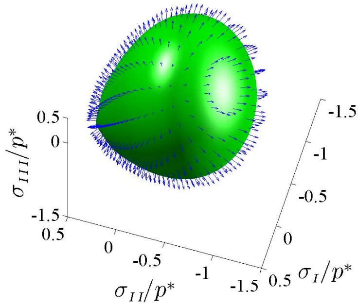
Fig. 7 Yield surface in dimensionless principal stress space decorated with flow vectors for a bonded granular assembly after kinematic hardening. View not down the hydrostatic axis. (See Table2 for parameter values: c = 0.5 ; v_r = 0.25 ; d_{ii}^g \neq 0 .)
