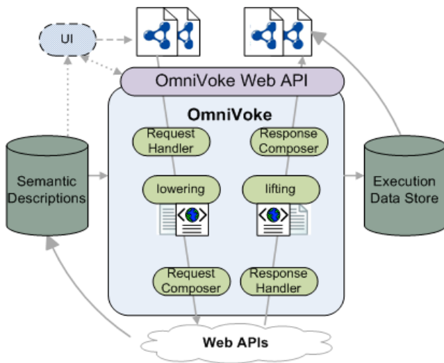
Figure 1. OmniVoke Architecture
