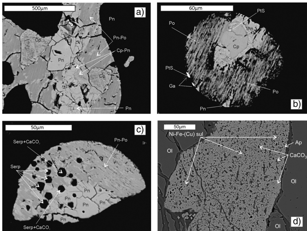
Fig. 6. Loch Roag xenolith SEM backscatter electron images (BSE). (a) Irregular-shaped 'complex sulphide' with granular pentlandite and cross-hatched chalcocopyrite which are texturally distinct from the surrounding pentlandite, pentlandite–pyrrhotite stockwork, and striated pyrrhotite. (b) Rounded 'droplet sulphide' showing pentlandite and chalcocopyrite have separated from striated pyrrhotite (with minor pentlandite flames). Discrete μm-scale platinum-group minerals occur within this high-PGE sulphide droplet. Pt-sulphide (probably cooperite) is within chalcocopyrite portion and at the margin of the droplet. Pt-sulphide at the droplet margin occurs with galena. (c) Spongy 'droplet sulphide' with partially serpentinised and Ca-carbonate filled inclusions. (d) Spongy apatite between olivine crystals. Note that the spongy texture is due to abundant rounded Ca-carbonate inclusions (dull 'holes' in apatite) as well as minor rounded Ni-Fe-(Cu) sulphide droplets as inclusions (bright spots). Mineral abbreviations are: olivine (Ol), serpentine (Serp), apatite (Ap), pentlandite (Pn), chalcocopyrite (Cp), pyrrhotite (Po), cooperite (PtS), galena (Ga), Ca-carbonate (CaCO 3 ).
