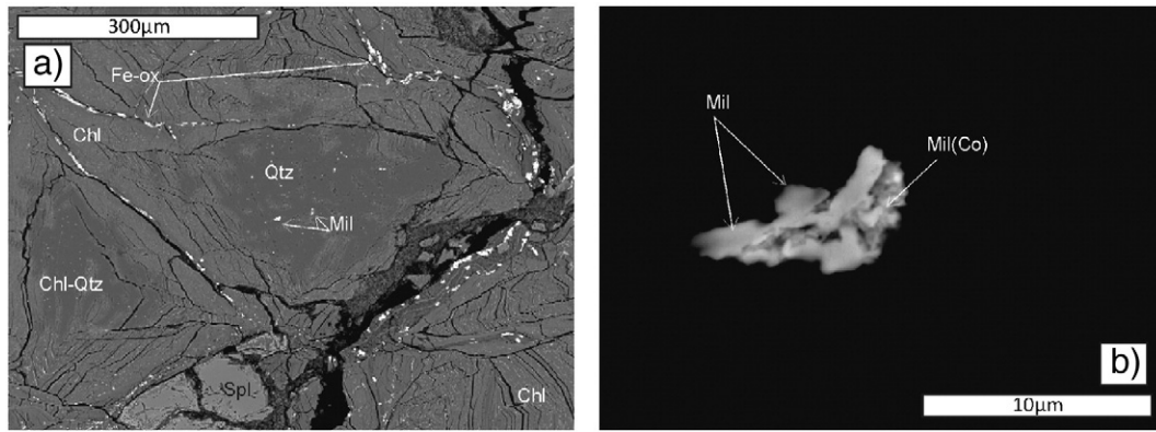
Fig. 10. Coire on Ba xenolith SEM BSE images. (a) Tiny millerite grains are inclusions in quartz. Quartz is intergrown with serpentine and chlorite (with accessory iron oxide). (b) Close-up image of a millerite grain, showing skeletal texture and areas of Co-bearing millerite (appearing brighter). Mineral abbreviations are: quartz (Qtz), serpentine and/or chlorite (Chl), iron oxide (Fe-ox), millerite (Mil), Co-bearing millerite (Mil(Co)).
