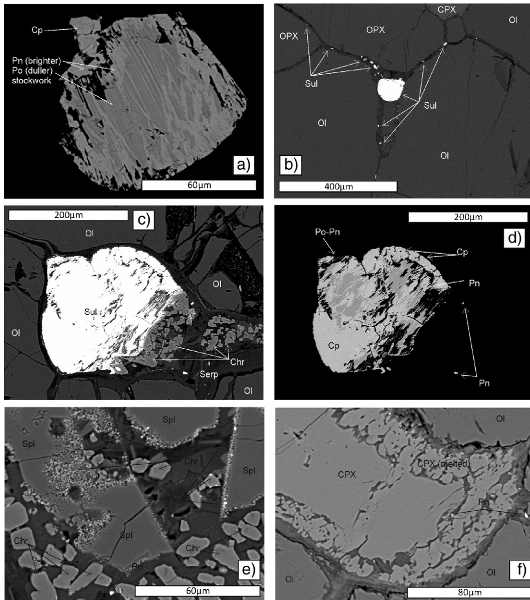
Fig. 8. Streak Com'laidh xenolith SEM BSE images. (a) Stockwork texture between pentlandite and pyrrhotite with minor chalcopyrite as distinct non-intergrown phases. Overall this is an example of a rounded sulphide globule. (b) Large rounded sulphide globule at olivine-orthopyroxene triple junction. Also note trail of \mu\text{m} -scale sulphides along silicate grain boundaries. (c) Sulphide at olivine grain boundaries (left) which is reacting on the right hand side to a more striated and irregular form. This reacting side is associated with fine-grained granular chromite within a pocket of serpentine. (d) The same sulphide as (c) with the contrast adjusted to display the sulphide internal texture and mineral phases. Note the rim of chalcopyrite vs. the central portion of intergrown pentlandite and pyrrhotite in a stockwork texture. (e) Al-Mg spinel melting at rim and forming granular chromite. Note the two crystal size populations of chromite: >5\ \mu\text{m} granular, sub-euhedral chromite crystals vs. \mu\text{m} -scale rounded chromites. Both chromite populations are associated with \mu\text{m} -scale pentlandite globules at crystal margins. (f) Protogranular clinopyroxene and olivine. Clinopyroxene is melting to form finger-like crystals at its margins. This melt zone is again associated with \mu\text{m} -scale pentlandite globules. Note that (e) and (f) also appear in Hughes et al. (2015b). Mineral abbreviations are: clinopyroxene (CPX), orthopyroxene (OPX), olivine (Ol), spinel (Spl), chromite (Chr), serpentine (Serp), pentlandite (Pn), chalcopyrite (Cp), pyrrhotite (Po).
