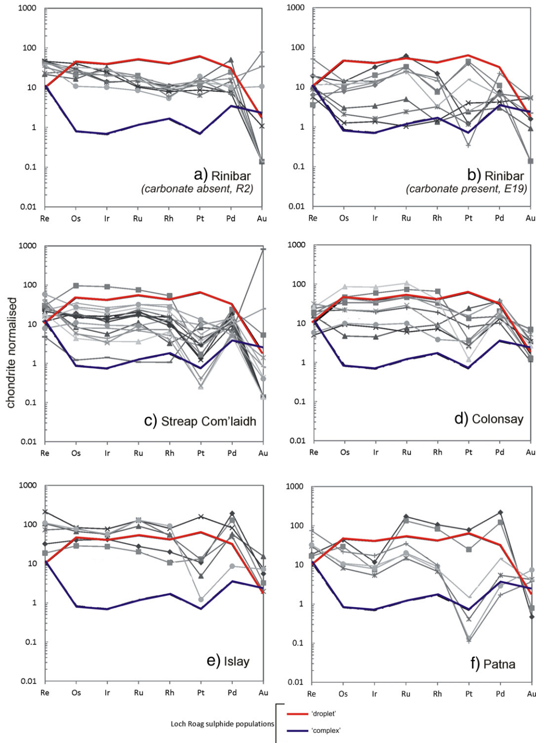
Fig. 12. Sulphide PGE multi-element diagrams per xenolith suite (chondrite normalised; McDonough and Sun, 1995): (a) Rinibar sulphides from carbonate-absent xenolith (sample R2), (b) Rinibar sulphides from carbonate-present xenolith (sample E19), (c) Strep Com'laidh, (d) Colonsay, (e) Islay and (f) Patna sulphides. All plots show mean sulphide compositions of 'complex' and 'droplet' sulphides from Loch Roag, for reference. LA-ICP-MS data.
