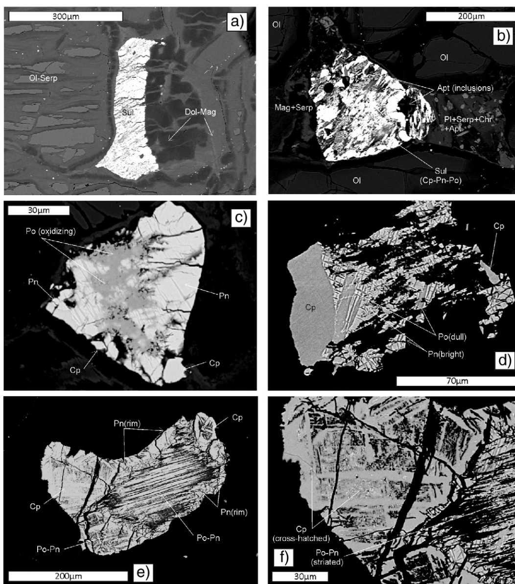
Fig. 7. Rinibar xenolith SEM backscatter electron images (BSE). (a) Elongate sulphide at the margin of a carbonate pocket and in contact with a serpentinised olivine crystal. Carbonates consist of intergrown dolomite and magnesite (sample E19). (b) Sulphide at the margin of a carbonate pocket (left hand side) and melt pocket (right hand side) inbetween granular serpentinised olivine crystals (sample E19). Carbonate pocket comprises magnesite, with minor serpentine probably entrained from the neighbouring olivines. The melt pocket consists of finely crystalline plagioclase, chromite and apatite, with accessory serpentine. Apatite inclusions occur within the sulphide globule. Sulphide minerals within the globule include chalcocopyrite, pentlandite and pyrrhotite. (c) Sulphide at silicate triple junction (sample R2) – carbonate is absent. Contrast adjusted to show two outer edges of intergrown chalcocopyrite and pentlandite with a central 'dappled' zone of pyrrhotite which is partially oxidising on the top left hand edge (sample R2). (d) Another example of a partially oxidising sulphide showing original chalcocopyrite and cross-hatched intergrown pentlandite and pyrrhotite, which now has a dappled, skeletal and 'frayed' appearance as a result of partial melting (sample R2). (e) Mixed base metal sulphide (sample R2) showing multiple and complex textures within the grain. Carbonate is absent from this sample. (f) Close-up of left hand side of sulphides in (e) showing cross-hatched and granular appearance of chalcocopyrite, next to striated pentlandite–pyrrhotite. Note the fine granular chalcocopyrite and pentlandite crystals in the lower right hand corner of this image. This exemplifies the multiple generations of sulphide crystal growth associated with an 'aggregate' of sulphides. Mineral abbreviations are: olivine (Ol), serpentine (Serp), clinopyroxene (Cpx), dolomite (Dol), magnesite (Mag), plagioclase (Pl), chromite (Chr), apatite (Ap), iron oxides (Fe-ox), orthoclase (Kfs), biotite (Bt), ilmenite (Ilm), pentlandite (Pn), chalcocopyrite (Cp), pyrrhotite (Po).
