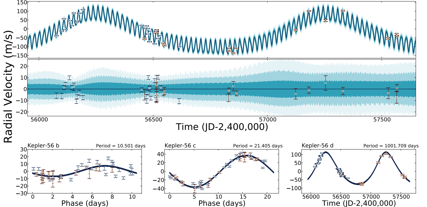
FIG. 1.— A suite of results from our MCMC fit. (Top) Kepler-56 RV data – with HIRES points in red and those of HARPS in navy – together with a curve whose gradient represents the differing confidence levels of MCMC’s results, with the darkest navy representing the median fit and lighter shades corresponding to the 1, 2, and 3\sigma uncertainties on the RV of the star as a function of time. (Middle) Identical to Panel 1, save that each data point and confidence curve has been subtracted by the median fit RV in order to show the data residuals and uncertainty as a function of time. (Lower left) Individual, phase folded RV contribution of Kepler-56 b to the system’s total RV. The contributions of the other two planets are subtracted from the HARPS and HIRES data displayed on the plot for visualization purposes. (Lower middle) The phase folded version of the lower left plot for Kepler-56 c with the signals from the other two planets removed for visualization purposes. (Lower right) Kepler-56 d’s individual, non-phase folded RV contribution, again with the other two planets removed.
