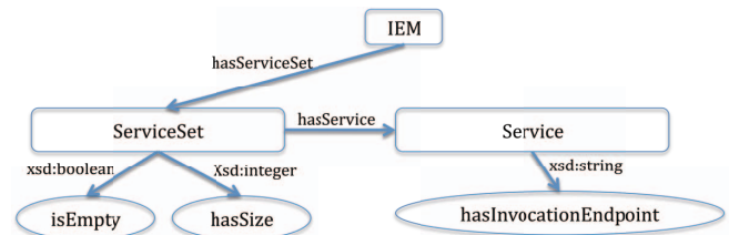
Figure 4. First-draft of IEM RDF schema
