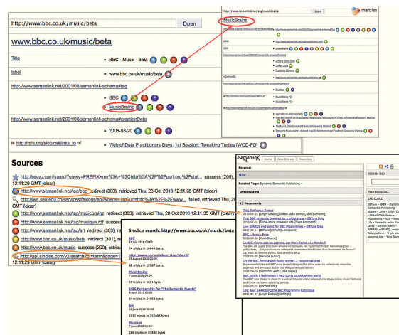
Fig. 11. The results of a request for the URI http://www.bbc.co.uk/music/beta are shown on the left. We then browse to the resource MusicBrainz (top, right). Two sources of information on the resource of interest ( BBC Music Beta ) are also retrieved from Sindice and Semanlink 46 (bottom, centre and right).
