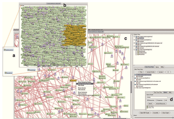
Fig. 20. Loading the URL http://www.bbc.co.uk/music/artists/a-z/by/a.rdf into RDF Gravity displays, first, the three concepts (from the MO) in the dataset – MusicGroup, SoloMusicArtist and MusicArtist (a). Loading the complete RDF graph (b) displays all instances of artists and groups whose names begin with ‘A’ (b). Even with a filter on labels to reduce occlusion (see far right), a very dense layout results. The central snapshot (c) zooms into the ROI (the nodes highlighted by selecting – yellow – in (b)) to display the links into and out of the node for the artist “Tina Arena” – see also the text query in (d) overlaid on the filters on the right.
