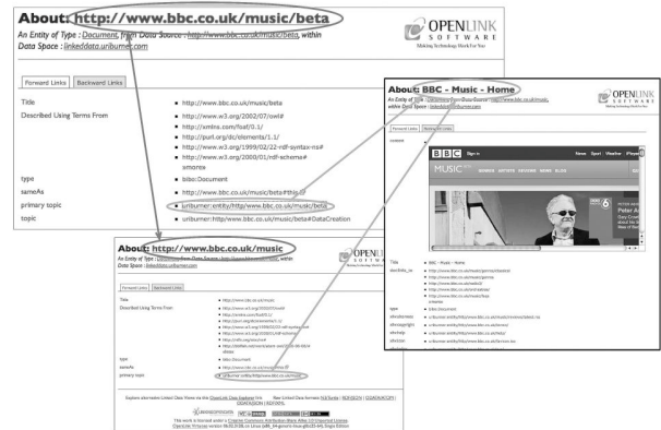
(a) Browsing from the resource URI for BBC Music Beta . On the right a template is used to display the result that includes the dereferenced URI (that retrieves the image) embedded in the output.
