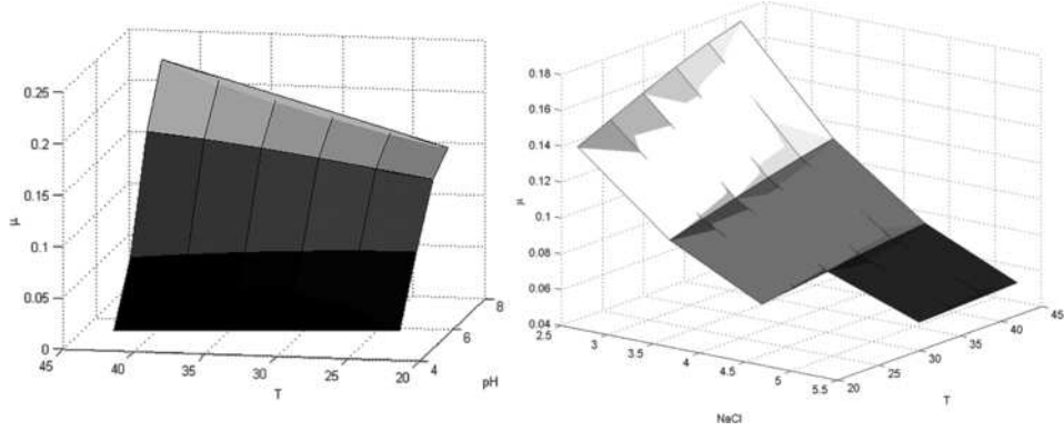
FIG. 6. Posterior mean of the growth rate parameter \mu for the GNN model. \text{NaCl} = 2.5\% (left) and \text{pH} = 6.5 (right).
