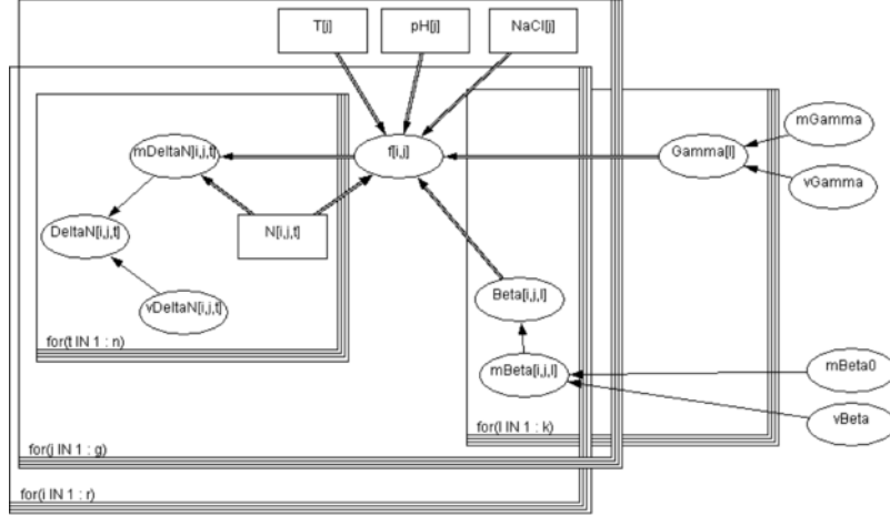
FIG. 4. Dependence structure of the NN model.
