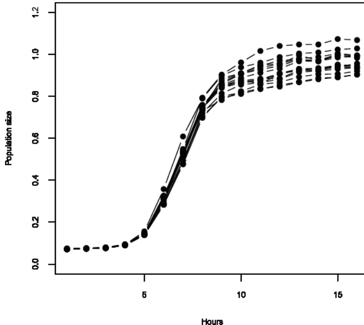
FIG. 3. 15 replications of bacterial growth under T = 42^\circ C , pH = 7.4 and NaCl = 2.5\% .
