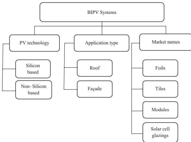
Fig. 4. BIPV categorization.
