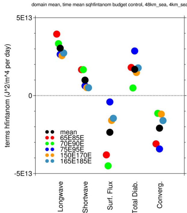
Figure 3. Daily mean values of domain-mean terms in the h^2 budget ( J^2 m^{-4} d^{-1} ) for control runs (sea points only) of each case. Note that x axis positions for each term vary slightly across cases for graphical clarity.
