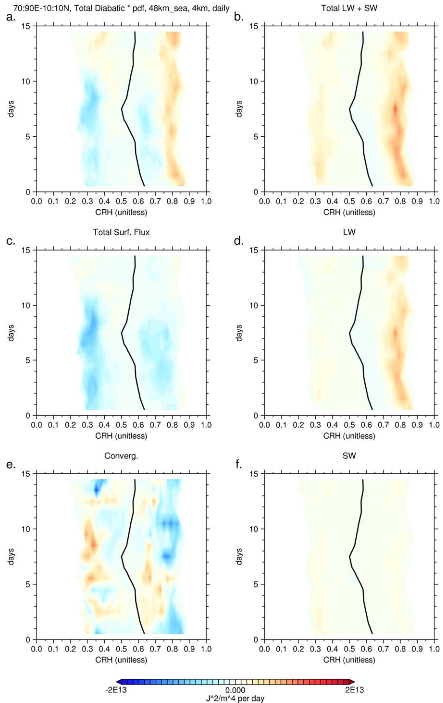
Figure 5. Daily mean values of 48 \text{ km} \times 48 \text{ km} blocks for terms in the \hat{h}^2 budget (sea points only) conditionally averaged by column relative humidity (CRH) for each day and multiplied by the probability density for that CRH and day, in units \text{J}^2 \text{ m}^{-4} \text{ d}^{-1} . The figures show (a) the sum of all diabatic terms, (b) the sum of contributions from longwave and shortwave radiation, (c) surface heat flux, (d) longwave radiation, (e) horizontal convergence of h flux, and (f) shortwave radiation; for the control run from 70^\circ\text{E} – 90^\circ\text{E} . The black line is the \hat{h}=0 contour.
