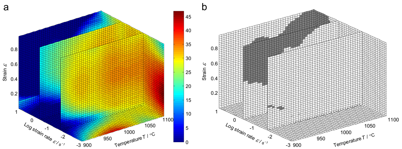
Fig. 8. (a) The 3D power dissipation maps and (b) the 3D flow instability map at strain rate 0.01, 1 and 10 s^{-1} .
