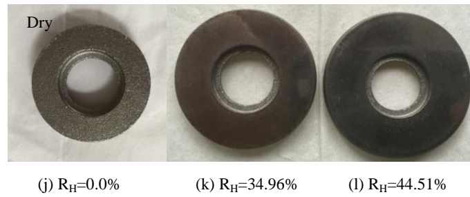
Fig. 10 The ring with inner boss after compression under different lubricating conditions
