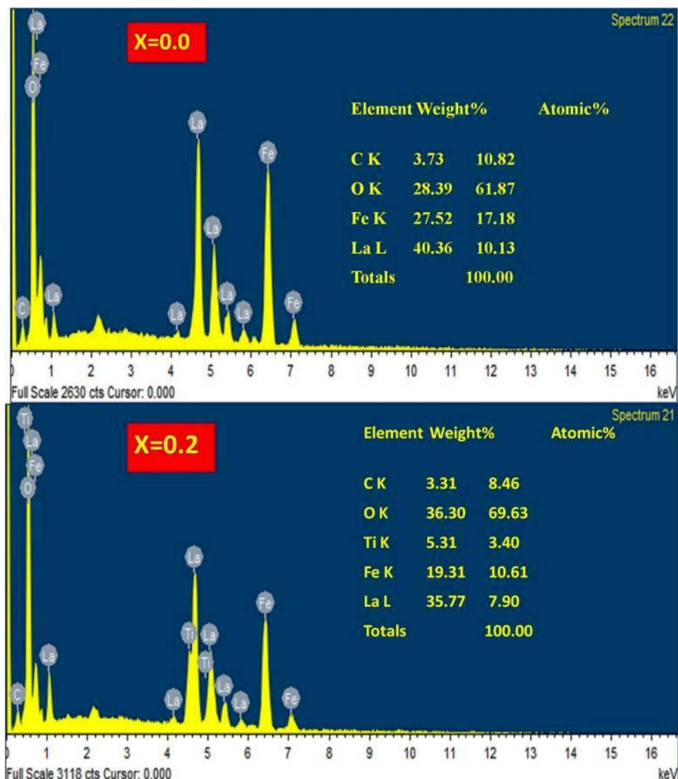
Fig . 3 EDAX spectra of \text{LaFe}_{1-x}\text{Ti}_x\text{O}_3 ( x = 0 & 0.2 )
