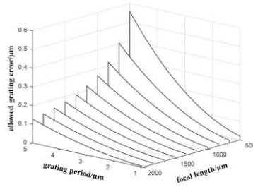
Figure 2: Allowed error in the grating period for the maximum central shift of 5 μm, assuming wavelength \lambda = 0.5 \mu\text{m}
