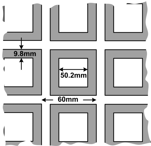
Fig. 1. Square-Loop FSS dimensions (substrate thickness: 1.6mm)
