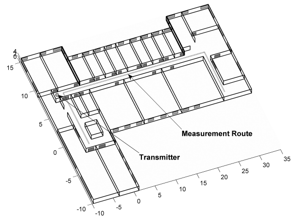
Fig. 9. Measurement route for validation of the Ray Tracing Tool
