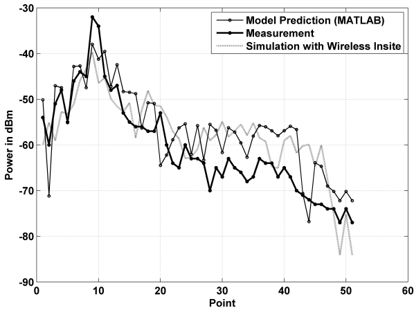
Fig. 10. Comparison between measurements and modeling
