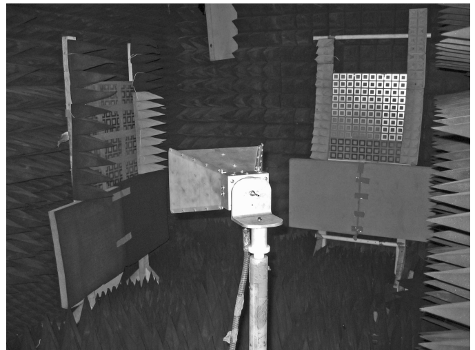
Fig. 12. Anechoic Chamber experiment setup
