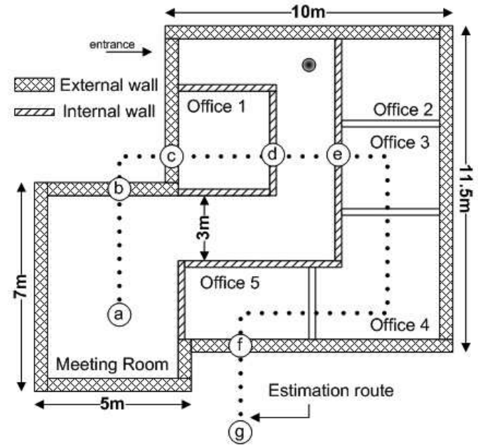
Fig. 14. Scenario under investigation (Height=3m)
