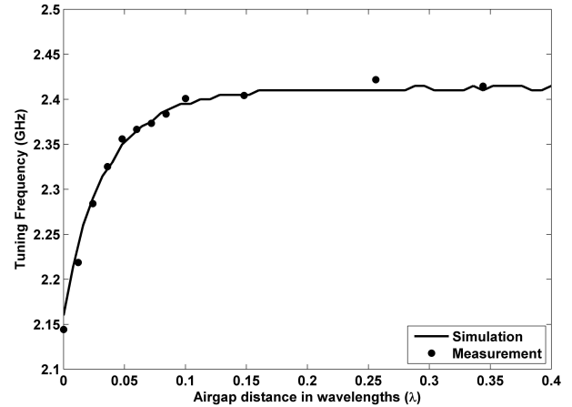
Fig. 8. Simulation and Measurement of the effect of the air gap between the square-loop FSS and a 9mm-thick wooden (MDF) board on the tuning frequency
