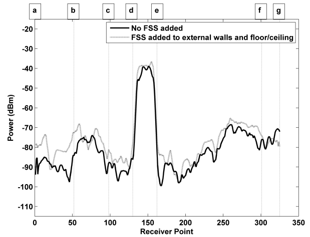
Fig. 17. Comparison of different cases at 5.2 GHz
