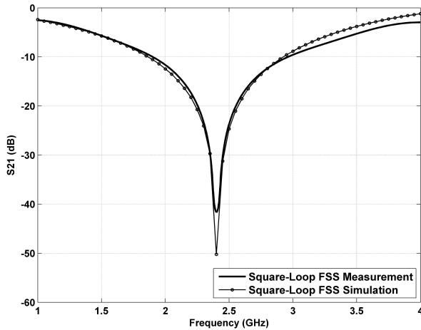
Fig. 3. Transmission through Square-Loop FSS at normal incidence
