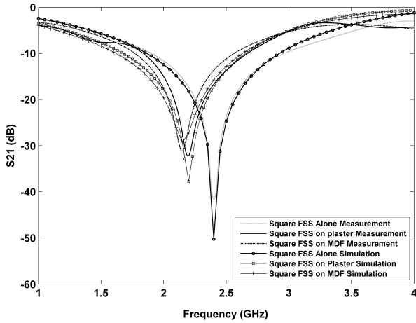
Fig. 6. Effect of wood and plaster when these are attached on the square-loop FSS
