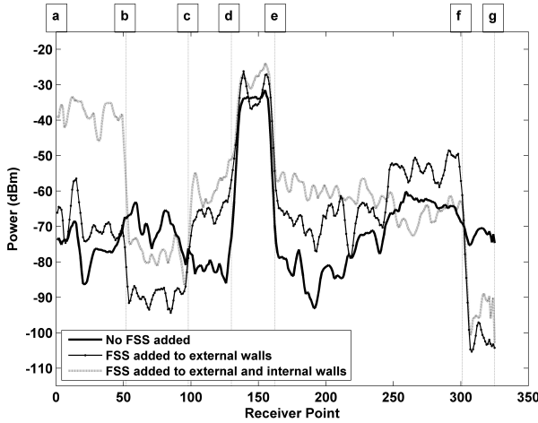
Fig. 16. Comparison of different cases at 2.4 GHz. The letters at the top of the figure correspond to the points along the estimation route shown as shown in Figure 14.
