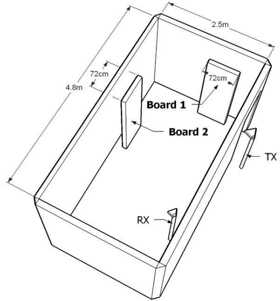
Fig. 11. Anechoic Chamber experiment setup
