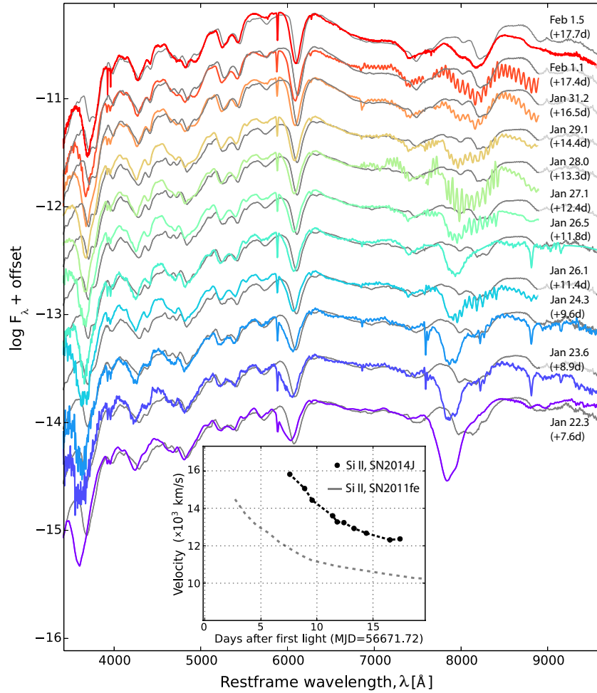
Figure 3. Pre-max spectroscopic follow-up of SN 2014J, starting 7.6 days from estimated supernova onset using the ARC 3.5 m DIS, LCOGT FLOYDS, NOT ALFOSC, and P200 DBSP spectrographs. Spectra of SN 2011fe (Pereira et al. 2013) at similar epochs (gray lines, reddened by E(B - V)_{\text{host}} = 1.2 mag with R_V = 1.7 and E(B - V)_{\text{MW}} = 0.14 mag with R_V = 3.1 are shown for comparison). The inset panel shows that SN 2014J has higher Si II velocity than SN 2011fe and a steeper velocity gradient (Benetti et al. 2005).
