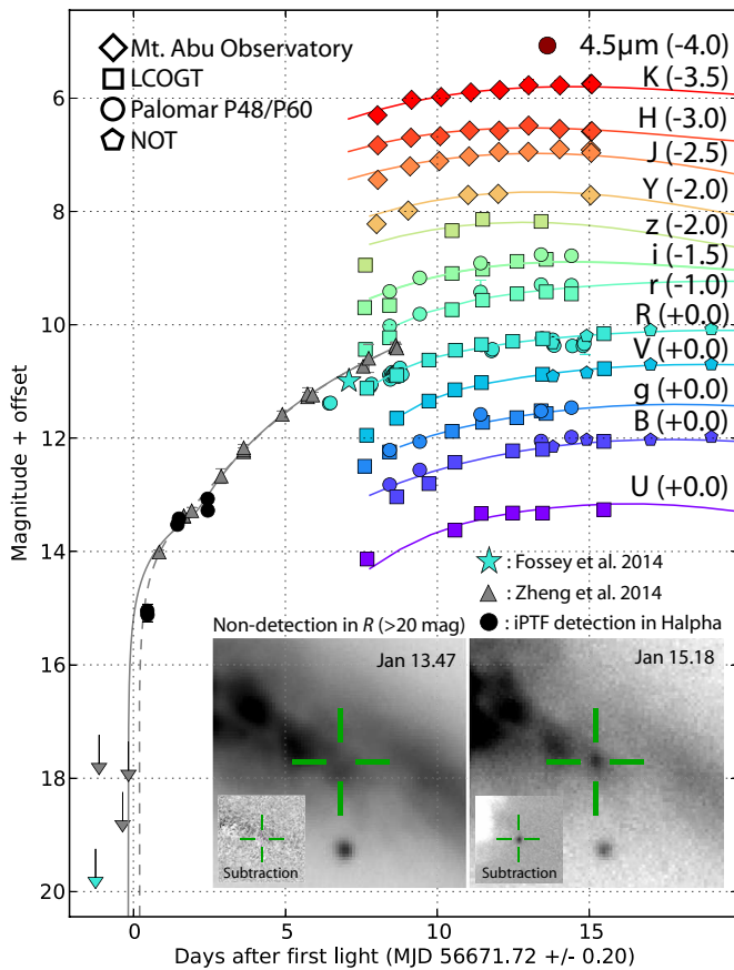
Figure 2. Light curves showing the rise of SN 2014J, along with SNooPy fits described in the text. The first P48 H_{\alpha}^{656} and H_{\alpha}^{663} narrowband detections are shown (black circles and inset image), S-corrected (Stritzinger et al. 2002) to the R band. Due to lack of accurate absolute calibration for the H_{\alpha} filters, a common offset was applied to connect with the data points in the pre-discovery light curve presented in Zheng et al. (2014). We also show their two fits to t_0 , suggesting our first detection could be within \sim 5 hr from the onset of the supernova.
