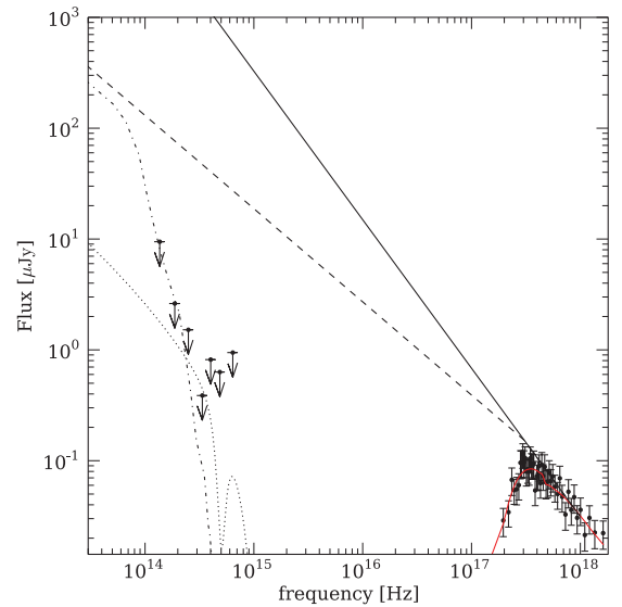
Figure 2. The afterglow SED \sim 11 h post-burst, ranging from nIR to X-ray frequencies. The solid red line shows the X-ray model fitted with redshift z = 1.74 , the solid black line is the X-ray power law extrapolated without a spectral break and the dashed line with a \Delta\beta = 0.5 cooling break. The power law and spectral break model is shown absorbed in the rest frame by a MW reddening law with A_V = 2.6 (dotted line), and by a SMC law with A_V = 3.7 (dash-dotted line).
