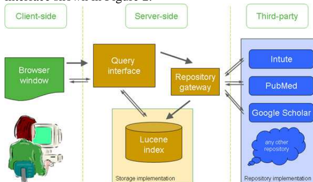
Figure 1: Architecture of DYNIQX
