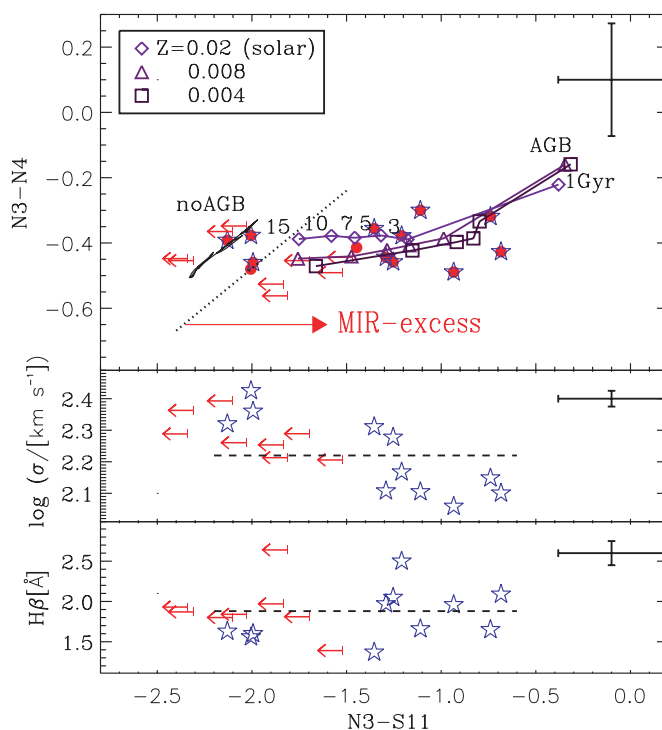
Figure 2. Top: the N3 - N4 vs. N3 - S11 color-color diagram for galaxies in the box of Figure 1(b). Symbols have the same meanings as Figure 1(c). The diamond, triangle, and square symbols represent loci of the P03 AGB models along mean stellar ages (1, 3, 5, 7, 10, and 15 Gyr) for Z = 0.02 (solar metallicity), 0.008, and 0.004, respectively. The thick solid line shows the P03 noAGB model color. MIR-excess galaxies as those redder than dotted line in N3 - S11 ( 1\sigma redder than the P03 noAGB model). The cross represents the median errors. Middle: the velocity dispersion vs. N3 - S11 color for Z01 data available. Symbols as the upper panel. The dashed line represents the mean value of \sigma for 48 ETGs in Z01. Bottom: H\beta line index vs. N3 - S11 color for Z01 data available. Symbols as the upper panel. The dashed line represents the mean value of H\beta line indices for 48 ETGs in Z01.
