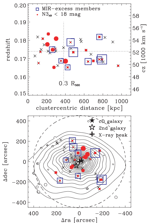
Figure 4. Upper: the cluster-centric distance and velocity distributions for the 39 A2218 AKARI cluster ETGs (“x” symbols). The filled circles are ETGs with N3 < 18 mag, and the size is proportional to N3 flux. The squares are MIR-excess galaxies as defined in Figure 2, and the size is proportional to F_{11}/F_3 flux density ratios (mass-normalized MIR excess). The vertical dotted line indicates the radius to divide into two bins and R_{500} is usually known as roughly half of the virial radius (1.21 Mpc from Maughan et al. 2008). Lower: the spatial distribution overlaid with the adaptively smoothed X-ray contours adopted from Maughan et al. Symbols as the upper panel. The cross, the filled star, and the open star indicate the position of the X-ray brightness peak, the cD galaxy, and the second brightest cluster galaxy, respectively. The dashed circle corresponds to the radius R_{500} .
