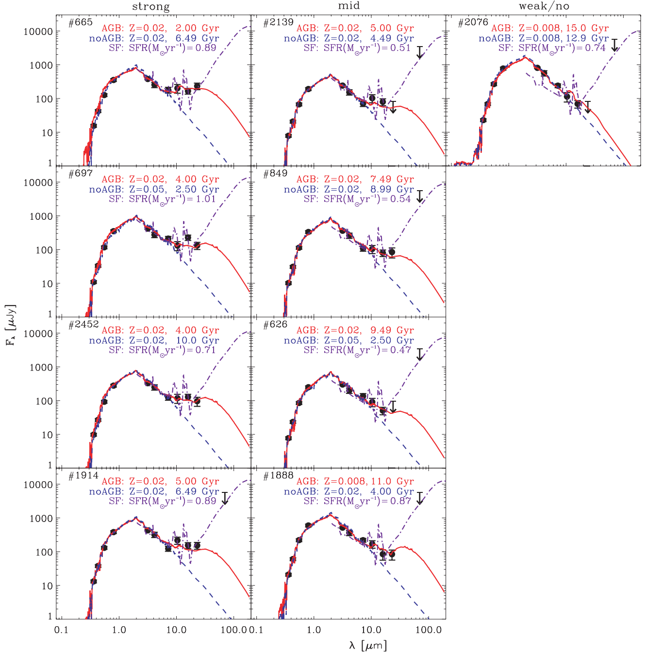
Figure 3. Observed SEDs of the S11-detected galaxies with Z01 optical and the Spitzer 24/70 \mu\text{m} data available. The best-fit lines of three different models (AGB: solid; noAGB: dashed; SF: dashed-dotted) are overlotted with 1\sigma error bars. The arrows represent the 3\sigma detection limit.
