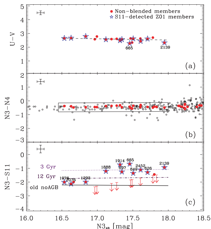
Figure 1. Top: the U-V vs. N3 CM diagram for N3 flux limited ETGs. The filled circles indicate our nonblended ETGs, and among them Z01 members detected in S11 are represented by star symbols. The galaxy numbers (No. 665 and No. 2139) are the notation used by Z01. The dashed line represents the best-fit U-V vs. N3 CM relation. The cross in the upper left corner indicates the median errors. Middle: the N3 - N4 vs. N3 CM diagram of AKARI IRC imaging sample. The open circles are all sources detected in the 15 \times 15 arcmin 2 field. Due to the detection limit of the S11 flux, we select bright ( N3 < 18 ) sources. Bottom: the N3 - S11 vs. N3 CM diagram for the galaxies in the box of panel (b). The 3\sigma detection limit are given for sources undetected in S11 (arrows). The dotted and the dashed-dotted lines indicate the CM relation calculated from the P03 AGB model SEDs assuming the metallicity gradient at two different stellar ages (3 and 12 Gyr), respectively. The solid line represents the 12 Gyr P03 noAGB model, assuming the metallicity sequence that fits the U-V vs. N3 CM relation.
