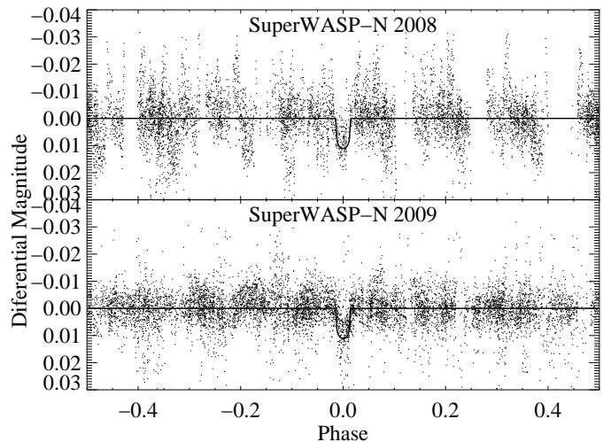
Fig. 1. SuperWASP phase folded light curve for WASP-38. On the top panel we show the 2008 data and on the bottom we show the 2009 data after the upgrade.
