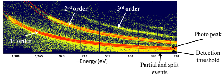
Figure 2. Energy vs. position plot for the XMM RGS camera array showing multiple orders demonstrating relatively low SNR for low energy photons.
