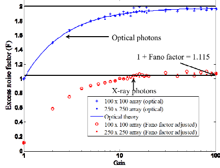
Figure 6. Plot showing the data obtained from the Monte Carlo model in an EM-CCD for X-rays (Fano factor adjusted and excess noise – bottom line) and optical photons (top line). The theoretical model for optical photons is also shown.
