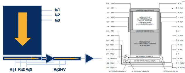
Figure 3. EM-CCD shown with parallel clocks ( I\phi ), serial clocks ( R\phi ) and High Voltage clocks ( R\phi HV ) on the left and the schematic of the CCD97 that was used for this work on the right [4] .
