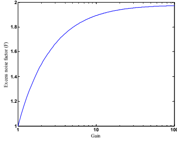
Figure 5. Plot showing the change in the excess noise factor (F) with varying gain.
