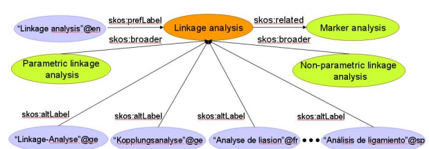
Figure 2: Representation of a concept linkage analysis in the multilingual ontology. The preferred label of this concept is the English version Linkage analysis . The concept has a two alternative representations in German ( Linkage-Analyse and Kopplungsanalyse ). 7 The representation in French is Analyse de liaison and in Spanish Análisis de ligamiento . The concept Linkage analysis is a broader concept for Parametric linkage analysis and Non-parametric linkage analysis , and it is related to a concept Marker analysis .
