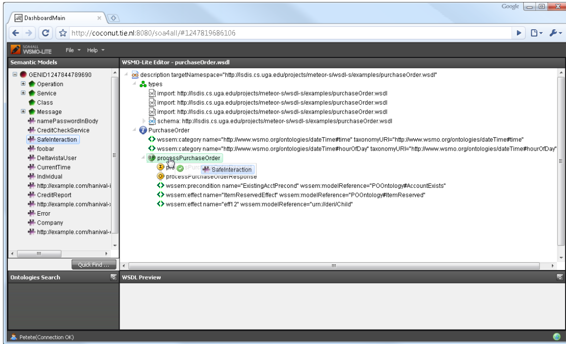
Figure 2. SOA4All Studio: WSMO-Lite Editor (Provisioning Platform)
