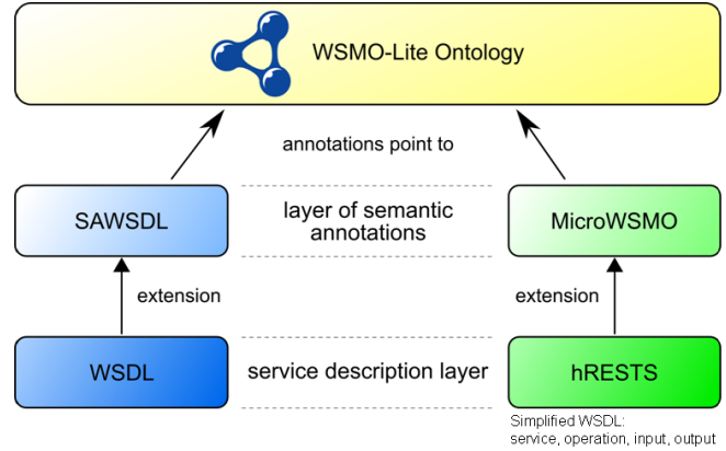
Figure 4. Lightweight service modeling overview
