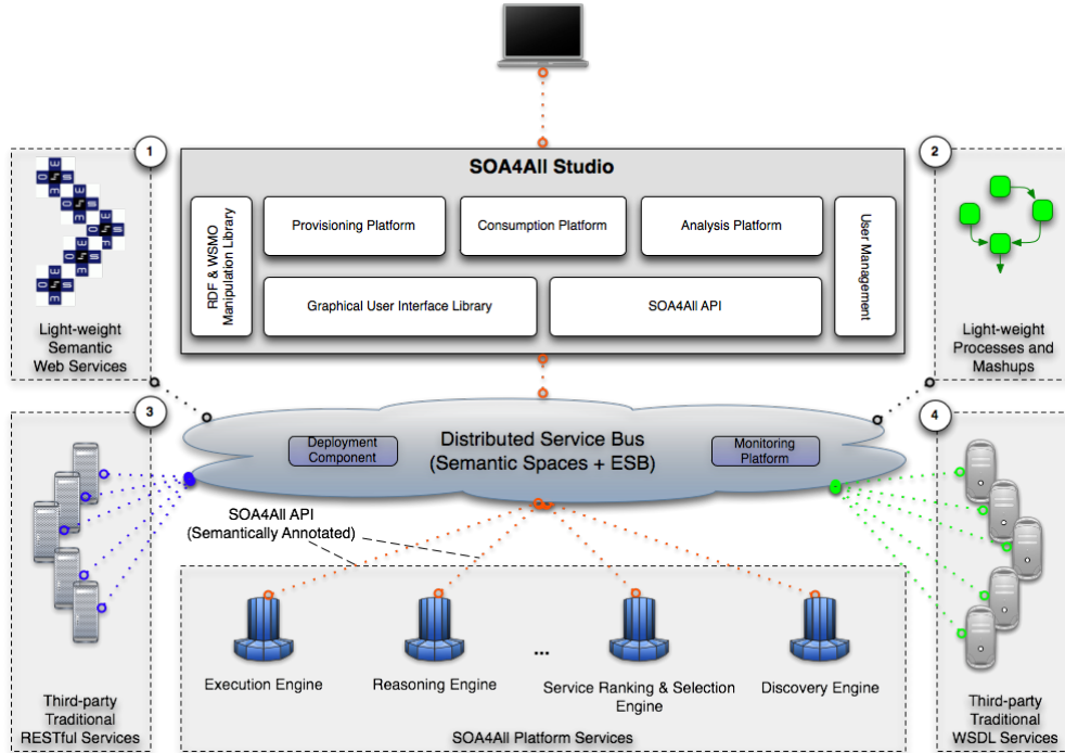
Figure 1. SOA4All overall architecture
