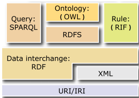
Figure 3. Four layers of the Semantic Web cake
