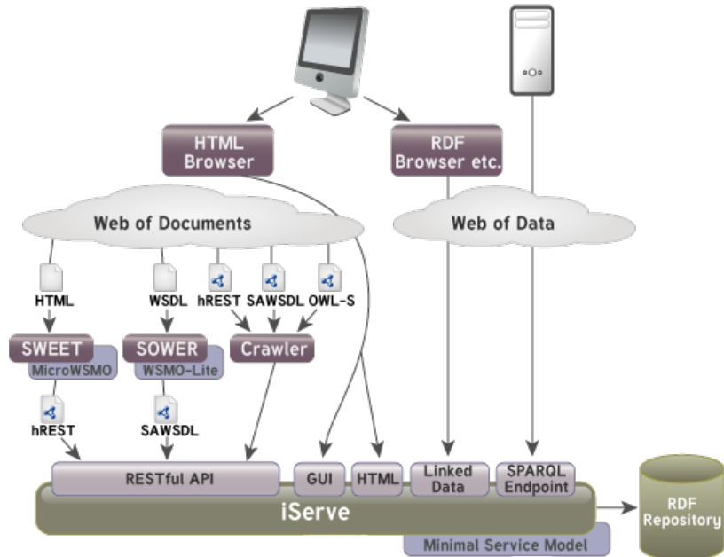
Figure 2: High-level architecture of iServe.
