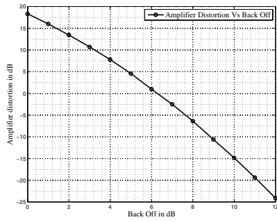
Fig. 2. Amplifier Distortion with Power BO
