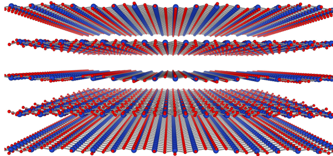
Fig. 1. An exaggerated illustration of a possible incommensurate modulation of \text{CuO}_4 planes (Cu in blue, O in red) such as found in the layered cuprate superconductors \text{La}_{2-x}\text{Sr}_x\text{CuO}_4 with parent I4/mmm symmetry. Although weak superstructure peaks have been measured that are associated with a charge density wave with a propagation vector \mathbf{k} = [0.23, 0, \frac{1}{2}] (Croft et al. , 2014), the limited number of weak observed reflections, the large number of possible isotropy subgroups, and the number of degrees of freedom within each of these models, means that the symmetry of the CDW phase in this and other related systems is still in question. The figure is drawn using ISODISTORT (Campbell et al. , 2006) and VESTA (Momma & Izumi, 2011).
