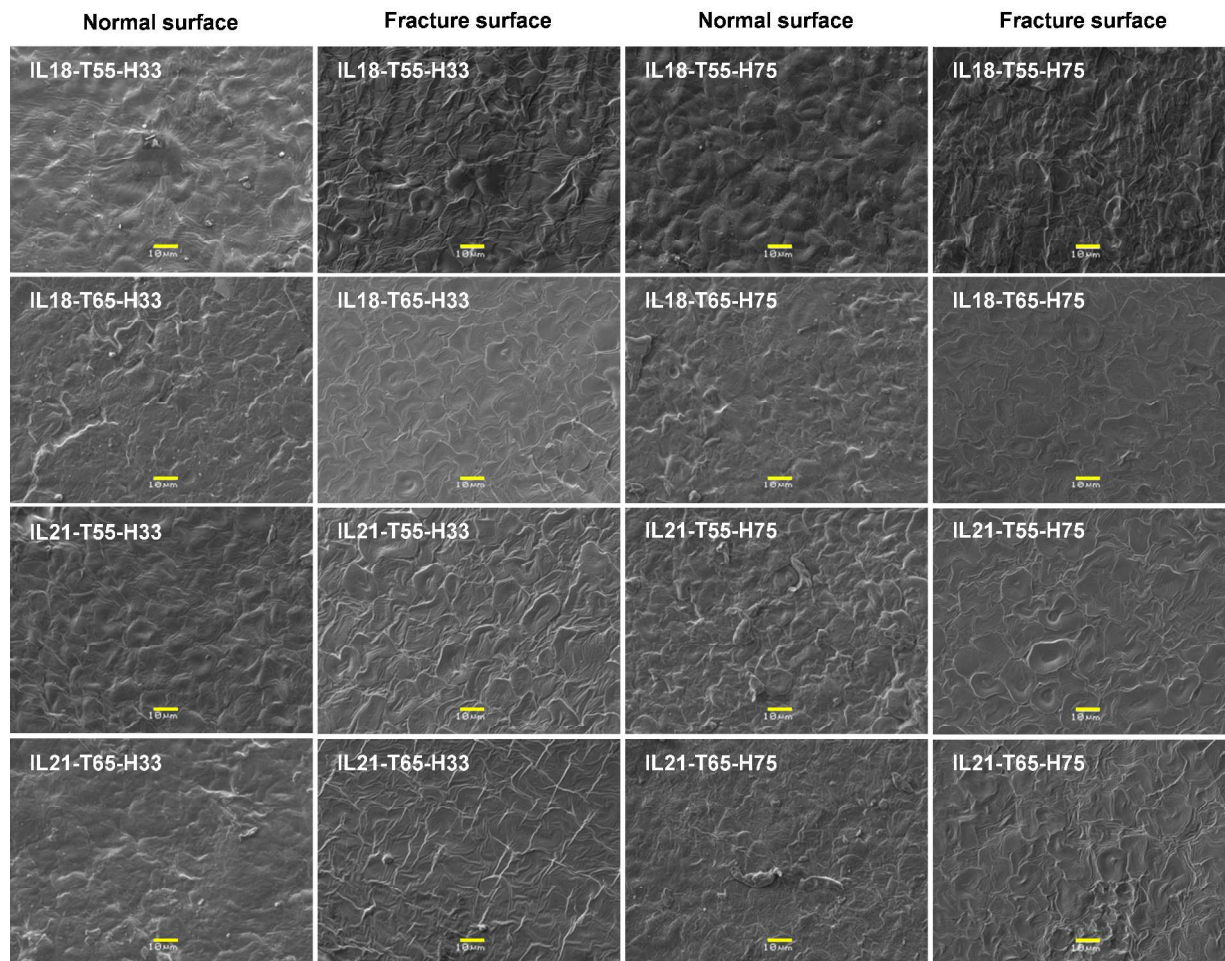
36 37 38 39 40 41 42 43 44 Figure 1. SEM images of normal and fracture surfaces of starch-[C 2 mim][OAc] films. The spot size was 6 nm. The scale bar (yellow) indicates 10 μm.
