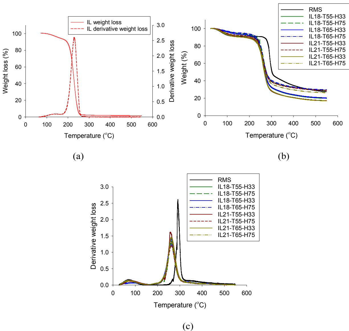
Figure 6. TGA results of the pure IL (a), and different starch-[C 2 mim][OAc] films (b, weight loss; c, derivative weight loss).
