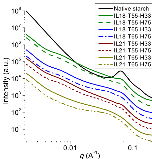
20 21 22 23 24 25 26 27 28 29 30 31 32 33 34 35 36 37 38 39 40 41 42 43 Figure 4. SAXS patterns for native starch and starch- [\text{C}_2\text{mim}][\text{OAc}] films. 44 45 46 47 48
