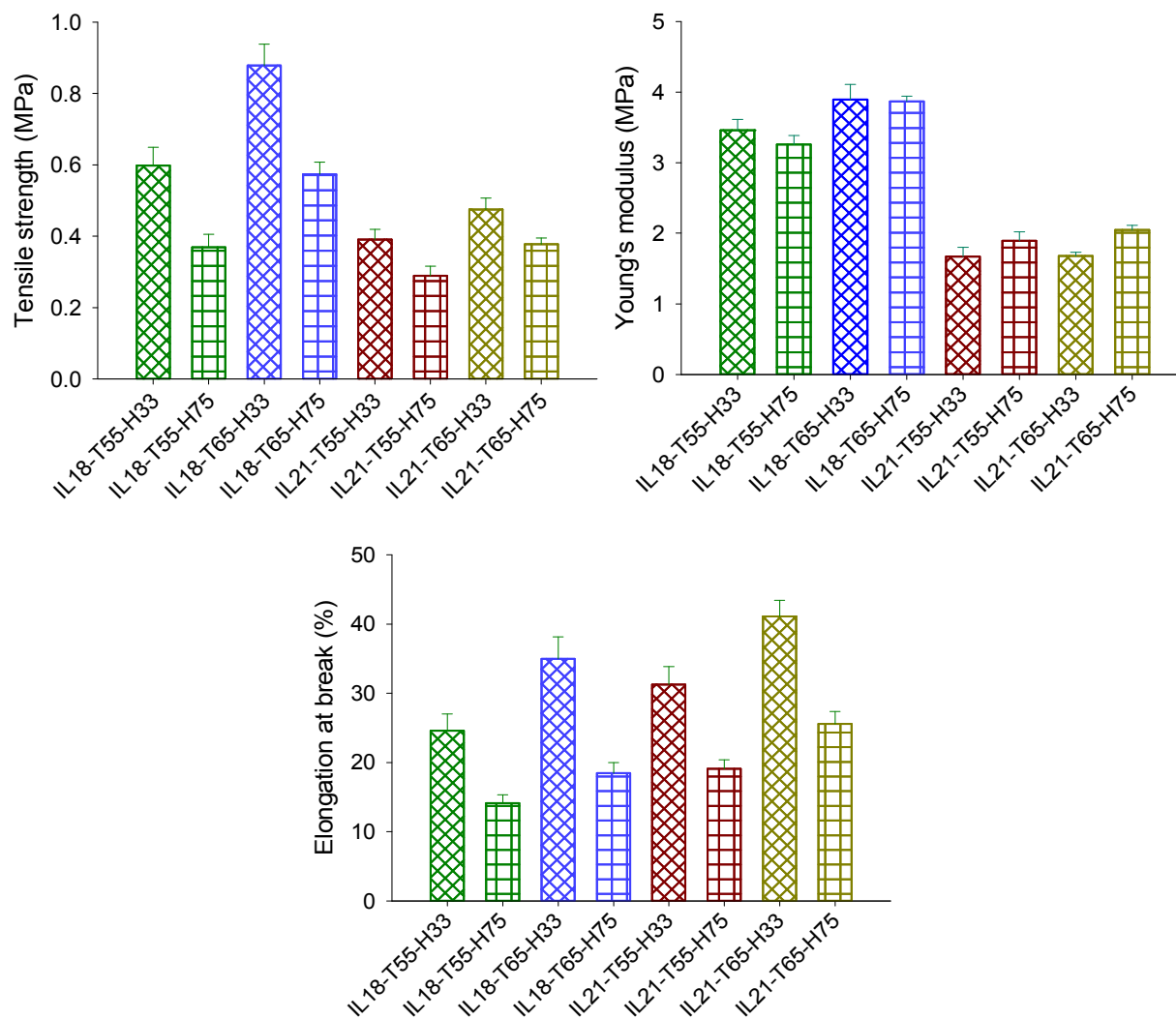
Figure 5. Tensile strength ( \sigma_t ), Young's modulus ( E ), and elongation at break ( \epsilon_b ) of starch- [\text{C}_2\text{mim}][\text{OAc}] films.
