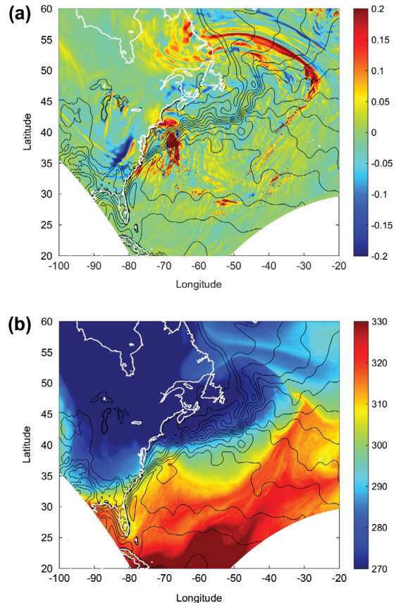
Fig. 2. Snapshots at t = 24\text{h} of (a) vertical velocity ( w , in \text{m/s} ) at z = 5\text{ km} and (b) equivalent potential temperature ( \theta_e , in \text{K} ) at z = 500\text{ m} . The corresponding surface temperature (=SST used in CNTL over the ocean) is shown in black with a contour interval of 2^{\circ}\text{C} , starting from 0^{\circ}\text{C} . The ‘white corners’ indicate the limit of the nested 12 km domain in that particular portion of the Northwest Atlantic.
