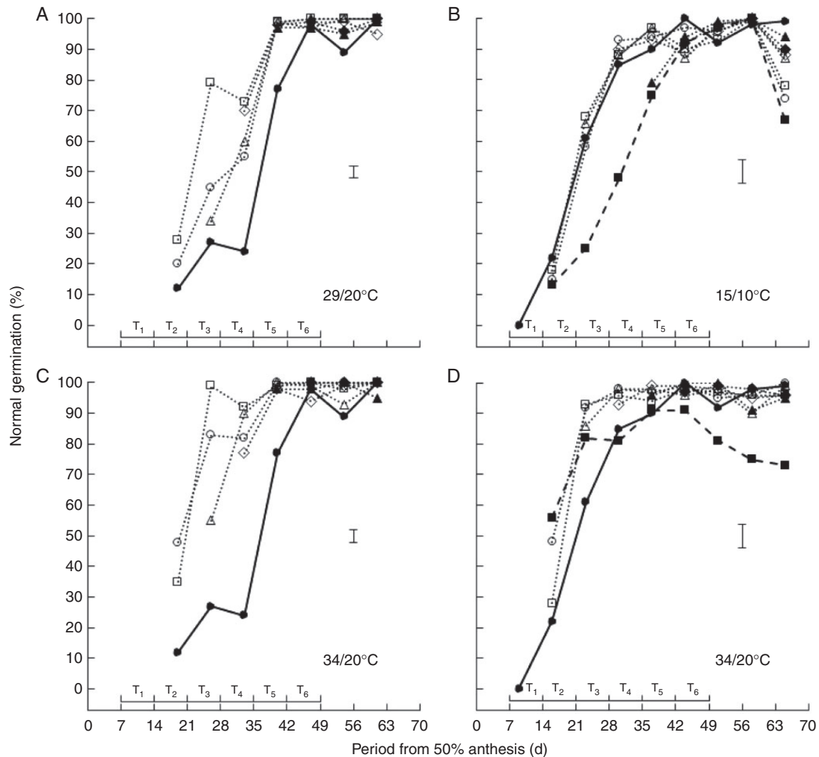
Fig. 4. Changes in ability to germinate normally of fresh seed of spring wheat 'Tybalt' control plants maintained at close to ambient temperature throughout (●) or exposed for different, successive 7-d periods from 7 DAA onwards to day/night temperatures of (A) 29/20 °C and (C) 34/20 °C (2010) or (B) 15/10 °C and (D) 34/20 °C (2011); T 1 (○), T 2 (□), T 3 (△), T 4 (◇), T 5 (▲), T 6 (◆). In 2011, treatments were also provided at 15/10 °C or 34/20 °C from 7 to 65 DAA (■). The horizontal bars represent the different 7-d periods (T 1 –T 6 ) when temperatures higher or lower than ambient were applied; vertical bars are least significant difference ( P = 0.05 ).
