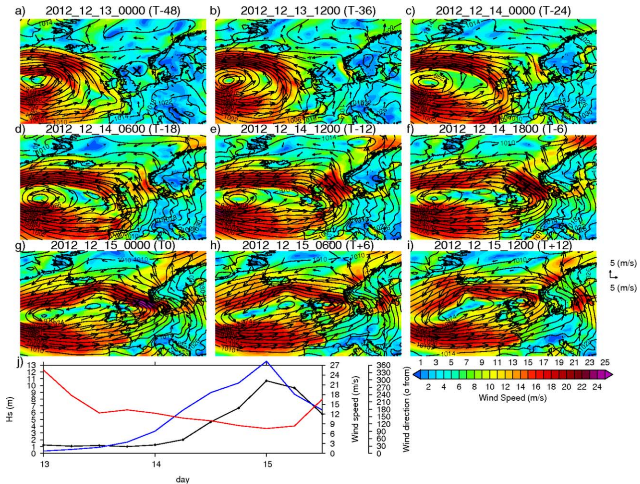
Figure 5. As for figure 4, but for synoptic evolution of the largest southerly H_s event (second largest H_s ) at Forties on 15 December 2012.
