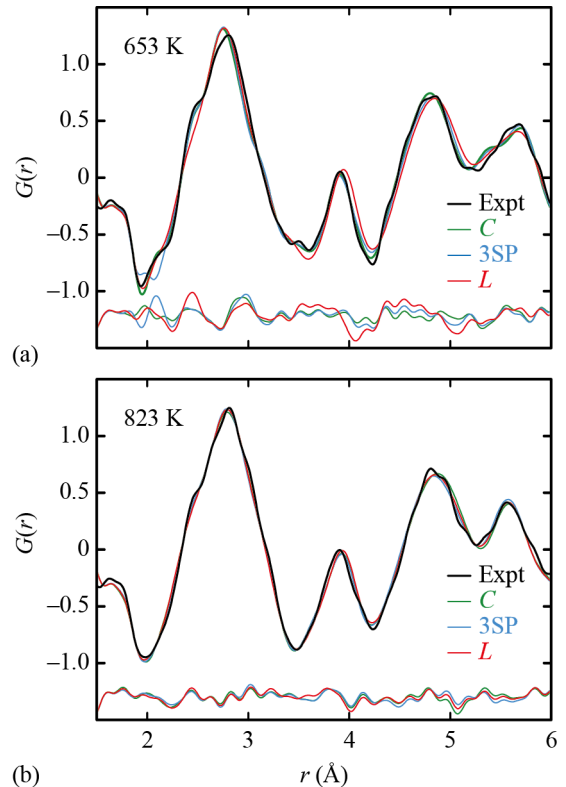
FIG. 6: Neutron PDF fits for data collected within the (a) O' and (b) O regimes. Experimental data are shown as black lines, and fits shown in green ( C -type order), blue (3SP-type order) and red ( L -type order). The corresponding difference functions (data – fit) are shown in the relevant colour, shifted vertically by 1.25 units. The fits shown here were for PDFGui refinements involving simultaneous fits to X-ray PDFs (see SI).
