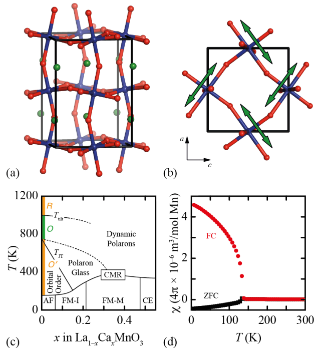
FIG. 1: Structure and phase behaviour of \text{LaMnO}_3 . (a) The ambient ( O' ) structure consists of a framework of corner sharing \text{MnO}_6 octahedra (Mn atoms blue; O atoms red), with La atoms (green) occupying 12-coordinate extra framework sites. The presence of octahedral tilts confers orthorhombic Pnma symmetry; in this representation the b axis is vertical and the c axis approximately horizontal. (b) Axial JT distortions are arranged with the same periodicity as the octahedral tilts. Long Mn–O bonds (indicated by arrows) are approximately confined within the (a, c) planes; this particular arrangement results in a small difference between the a and c lattice parameters. (c) On heating \text{LaMnO}_3 to T_{JT} = 750 K there is an isosymmetric structural transition to the orbital disorder ( O ) phase, with the same octahedral tilts as in the O' phase but with no discernible JT distortion. On hole doping, the value of T_{JT} decreases such that CMR emerges in \text{La}_{1-x}\text{Ca}_x\text{MnO}_3 from the disordered phase. A discontinuous octahedral tilt transition occurs at 1010 K to give a rhombohedral ( R ) phase that persists until decomposition. (d) Experimental d.c. magnetic susceptibility \chi for \text{LaMnO}_3 for the sample used in our study. The Néel temperature ( T_N ) is observed as a divergence in the field-cooled (FC) and zero-field-cooled (ZFC) traces at 140 K.
