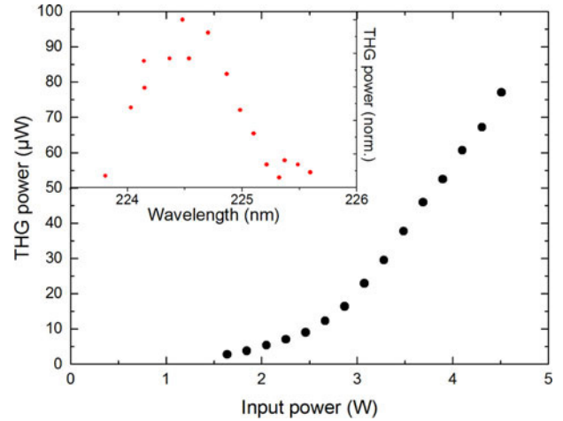
Fig. 4. Main: Third harmonic beam output power as a function of the pump power. Almost 78 \mu W of power is obtained at 224.5 nm. Inset: Normalised UVC output power of the laser as the wavelength is tuned by rotation of the birefringent filter. The tuning range is 350 \text{cm}^{-1} .
