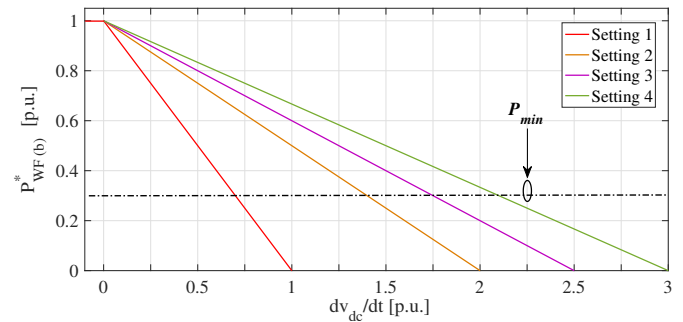
(b) Power curve settings
