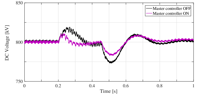
(b) DC-link voltage at T_2
