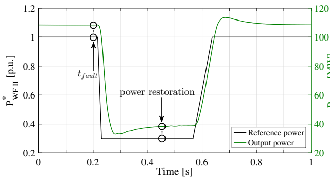
(c) Reference and output power for WF II
