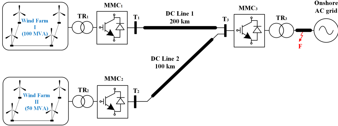
Figure 2: Wind farm integration using a three-terminal HVDC system.
