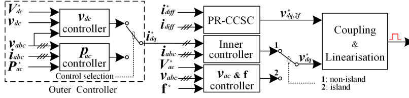
(a) Representation of the entire control structure of the MMC
