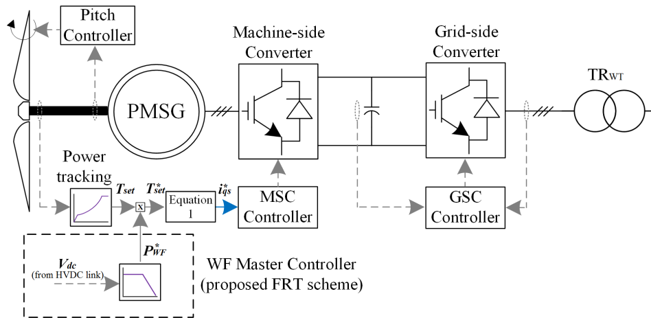
(a) Detailed schematic of PMSG and FRC
