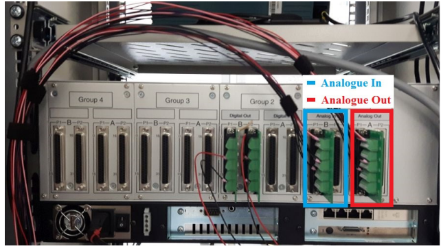
(b) OP5600 rear view
