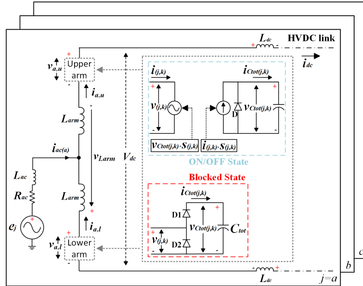
Figure 4: Detailed schematic with a three-phase equivalent of the MMC Type 3 model.
