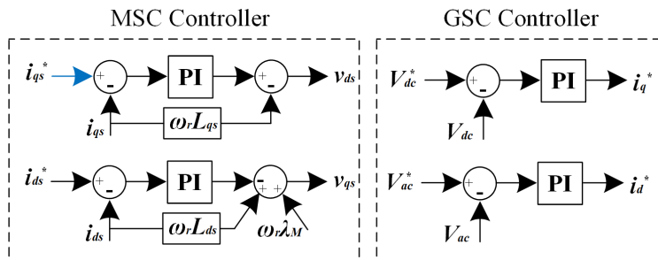
(b) Representation of the entire control structure of the FRC
