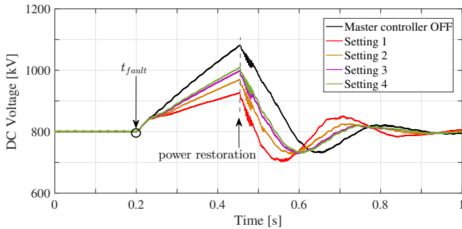
(a) DC-link voltages at T_1
