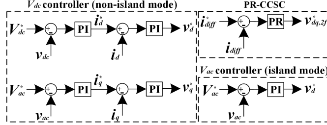
(a) Representation of the entire control structure of the MMC
