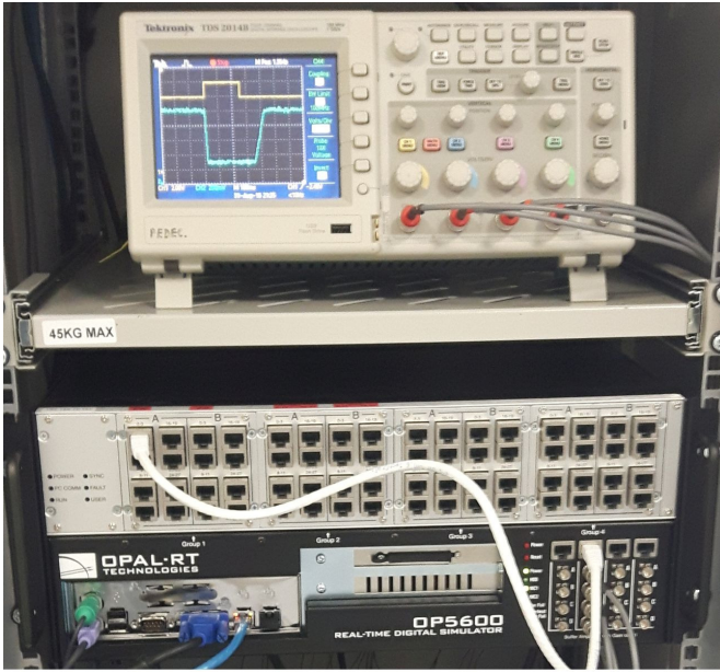
(a) OP5600 front view
