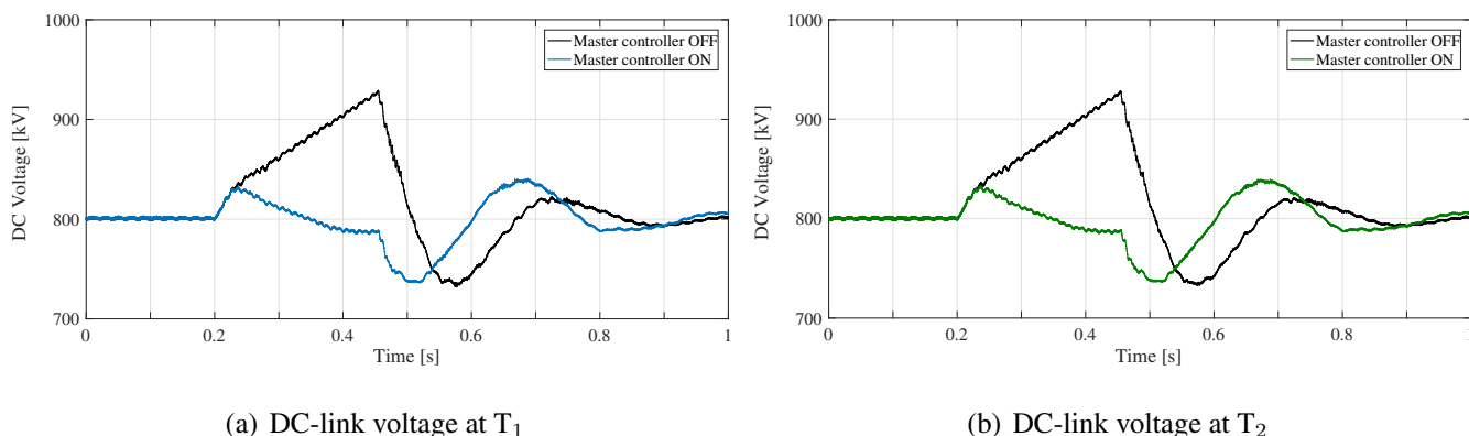
Figure 8: DC Voltage response for two-phase fault.
