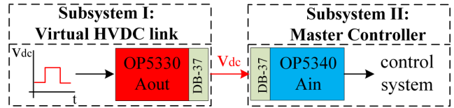
(c) Real-time model structure
