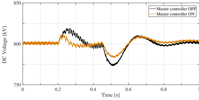
(a) DC-link voltage at T_1
