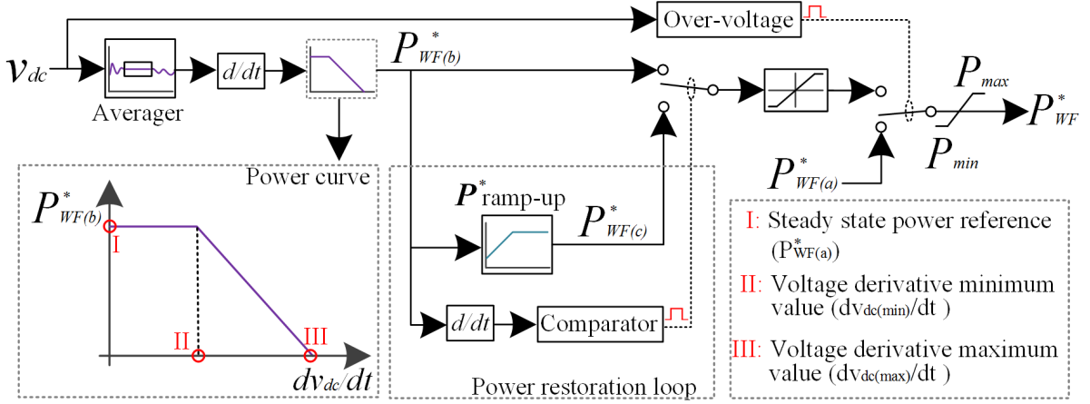
Figure 1: Master controller design.
