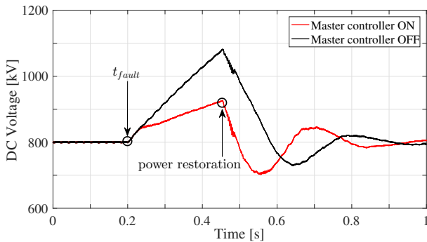
(a) DC-link voltage at T_2
