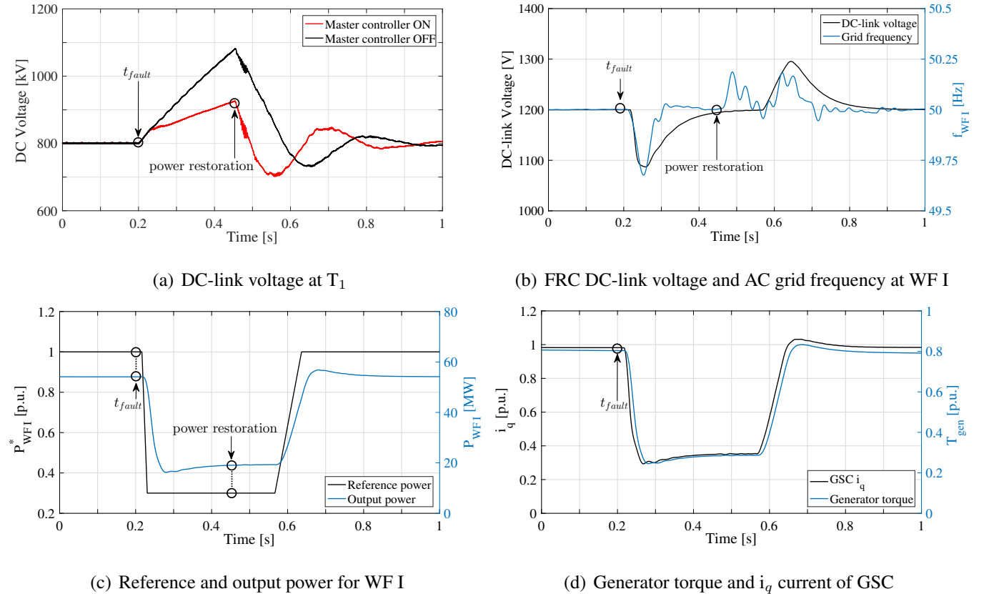
Figure 6: WF I response for a three-phase fault.
