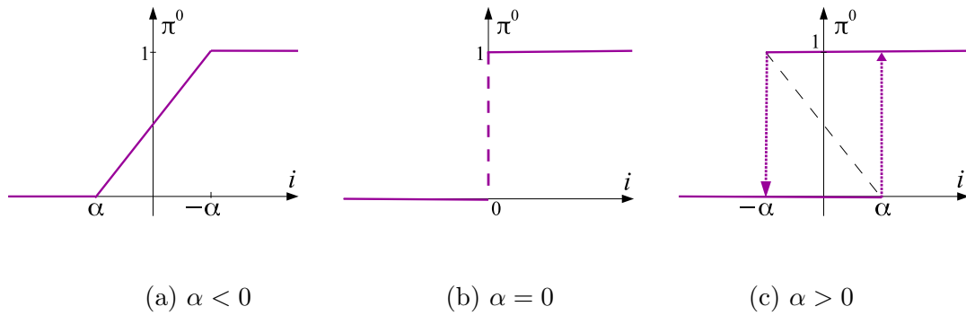
Figure 7. Response of model (5) to a slowly varying input i(t) in the limit when \gamma \rightarrow \infty and i'(t) \rightarrow 0 .
