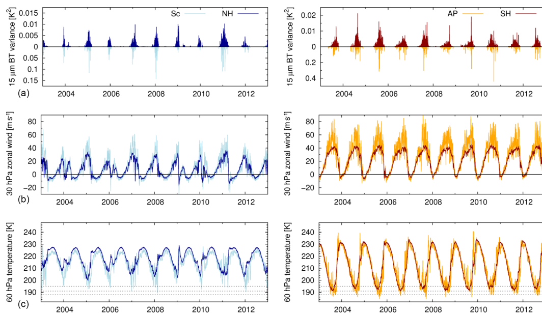
Figure 5. Time series of daily AIRS 15\ \mu\text{m} brightness temperature variances (top) as well as 6-hour ERA-Interim 30 hPa zonal winds (middle) and 60 hPa temperatures (bottom) at Northern Hemisphere mid- and high latitudes (NH; 55\text{--}85^\circ\text{N} ), the Scandinavian Mountains (Sc; 56\text{--}64^\circ\text{N} and 4\text{--}20^\circ\text{E} ), Southern Hemisphere mid- and high latitudes (SH; 85\text{--}55^\circ\text{S} ), and the Antarctic Peninsula (AP; 68\text{--}60^\circ\text{S} and 68\text{--}52^\circ\text{W} ). The dotted lines indicate typical PSC existence temperatures of T_{\text{ice}} = 188\ \text{K} , T_{\text{STS}} = 191\ \text{K} , and T_{\text{NAT}} = 195\ \text{K} at 20 km of altitude (Pawson et al., 1995).
