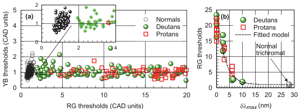
Fig. 3 YB thresholds plotted against the corresponding RG thresholds in 330 normal trichromats (black symbols), 269 deuterans (green symbols) and in 132 protans (red symbols) (a). A subset of deutan and protan subjects had full genetic analysis of their cone pigment genes and corresponding, \delta\lambda_{\max} values estimated. The black crosses in Figure 2c and d indicate the subjects selected for genetic analysis. The RG thresholds for these subjects are plotted against the corresponding \delta\lambda_{\max} values in Section (b). Note that according to these results, wavelength separations greater than some 15–20 nm yield ‘normal’ RG colour thresholds 4 (reproduced and modified from Barbur et al. 22 ).
