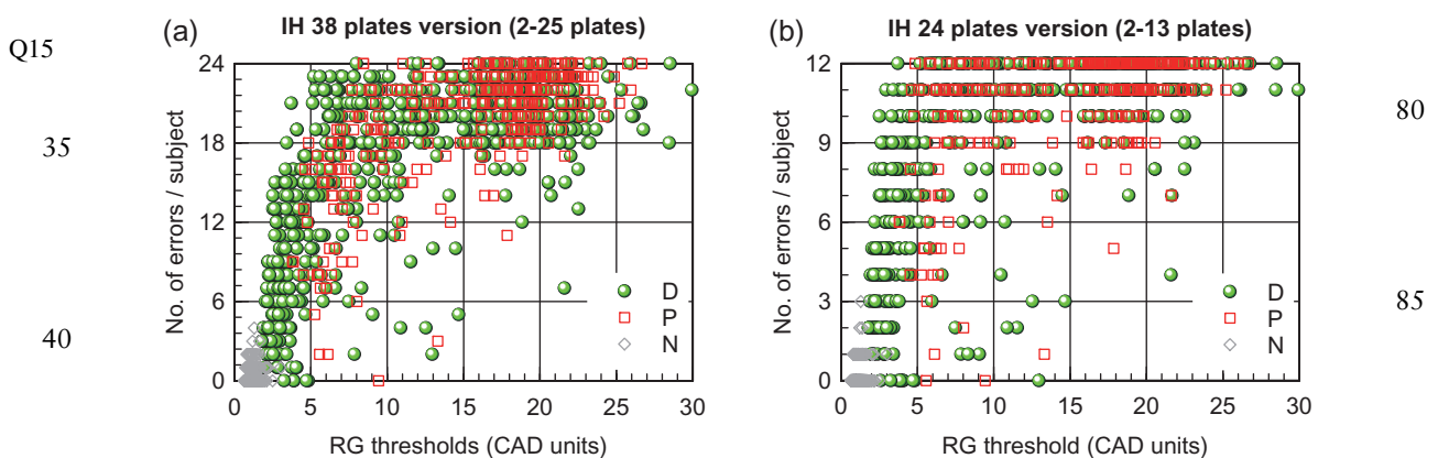
Fig. 10 The number of errors subjects make on Plates 2–25 of the IH-38 plates edition (a) and Plates 2–13 of the IH-24 plates edition (b). The latter is an efficient test because of the small number of plates involved and is used frequently in many industries with protocols based on two or fewer errors as a pass.
