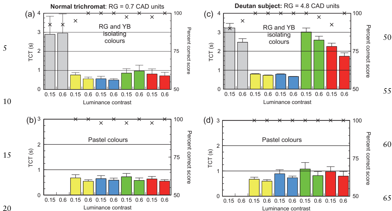
Fig. 14 TCTs with achromatic stimuli (grey bars) and when yellow, blue, green or red colours are added to the target. Data are shown for colours that isolate the RG and the YB chromatic mechanisms (a, c) and for 'pastel' colours that stimulate both RG and YB chromatic mechanisms (b, d). The deutan subject (with a RG threshold of 4.8 CAD units) requires longer TCTs for RG isolating stimuli, but performs as well as normal trichromats for the 'pastel' colours shown in Figure 15e. Percent correct scores are also displayed (black crosses) and reveal practically 100% correct scores in all the tests for both the normal trichromat and the deutan subject. Although the deutan subject requires longer TCTs when presented with RG isolating colours, he achieves 100% correct scores in all the tests.
