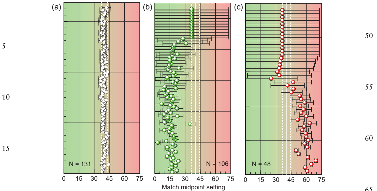
Fig. 12 The match midpoints are plotted in order of increasing matching range for normal trichromats (a) and for a number of deutan (b) and protan (c) subjects with varying severity of CV loss. The matching range is indicated by the horizontal bars that cross each midpoint. Dichromats can match the yellow field with any RG mixture. Some deutan and protan subjects exhibit very small matching ranges which suggests that although these subjects do not make normal matches, they are able to discriminate small changes in the RG mixture field as well as normal trichromats. (reproduced and modified from Barbur et al. 22 ).
