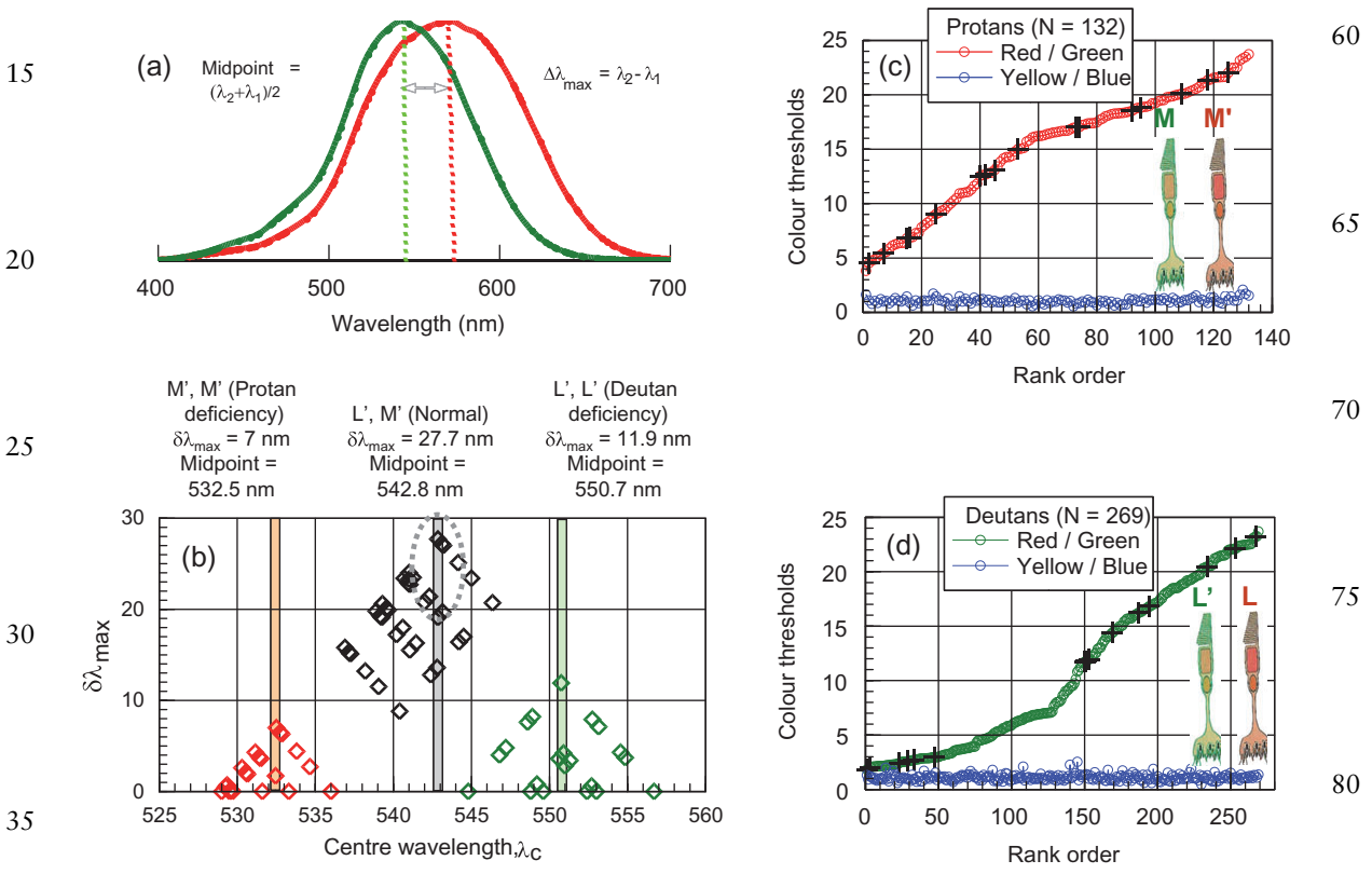
Fig. 2 The normalized spectral responsivity functions of L and M cones (a) reveal the wavelength separation, \delta\lambda_{\max} , and the midpoint between the two peaks. Both parameters affect chromatic sensitivity and the outcome of colour assessment tests. The 'potential' pairs of L- and M-cone pigment variants one can associate with a normal trichromat (black symbols), a deutan (plotted as green) and a protan (red symbols) observer (b). Note that for the same wavelength separation, \delta\lambda_{\max} , a protan and a deutan subject may perform quite differently in the same visual task. The RG and YB threshold colour signals measured in 132 protan subjects and ranked in increasing RG threshold are shown in (c). Note that a protan subject relies on a 'normal' M cone and a variant M' cone pigment which substitutes for the missing L pigment. The opposite is the case for deutan subjects. The graphs (c and d) illustrate the severity of RG CV loss which ranges from close to normal thresholds to complete absence of CV. The colour thresholds are measured in standard normal (SN) Colour Assessment and Diagnosis (CAD) units 3 which are described and illustrated in Figure 6. One CAD unit represents the mean threshold colour signal measured in 330 young, healthy normal trichromats. The CAD units are shown as arrows in Figure 6a together with the age distribution of the subjects (Fig. 6f) and the spread in RG and YB thresholds measured in this group (Fig. 6d and e).
