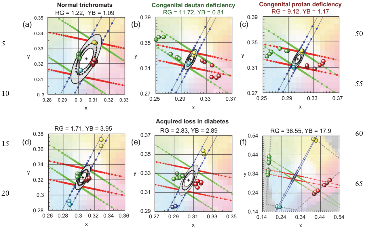
Fig. 8 Typical CAD thresholds are shown in (a) for a normal trichromat and in (b) and (c) for a subject with deutan- and protan-like congenital deficiency. The corresponding CAD thresholds for RG and YB CV are shown above each graph. Subjects with various degrees of loss of RG and YB chromatic sensitivity that are linked to diabetes are shown in (d), (e) and (f).
