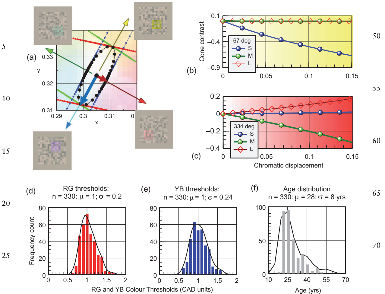
Fig. 6 RG and YB isolating axes are shown together with the threshold colour ellipse based on the mean RG and YB thresholds measured in 330, young, normal trichromats (d) and (e). The age distribution of the subjects is shown in Section (f). The minor and major axes of this ellipse define the SN CAD observer for RG and YB CV (see red and blue arrows in (a)). The screen dumps show the corresponding RG and YB isolating colours. Displacements away from background chromaticity along the YB and RG axes generate cone contrasts that are selective for S cones (b) and L and M cones (c). The larger these displacements, the more saturated the perceived colours. The measured thresholds are therefore directly proportional to the cone contrasts generated by the coloured stimulus.
