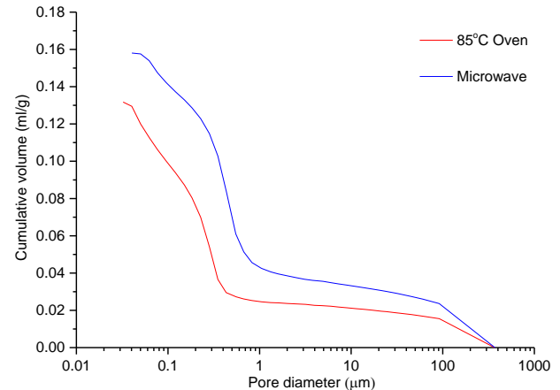
Fig. 4 Pore size distribution of hardened AAFA under thermal oven curing and microwave curing
