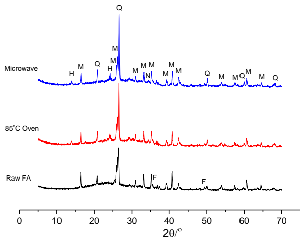
Fig. 2 XRD patterns of raw fly ash and AAFA under thermal curing and microwave curing (Q-quartz, M-mullite, F-hematite, H-hydroxysodalite, N-chabazite-Na)
