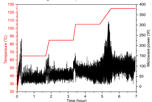
Fig. 1 Temperature profile and power profile of AAFA sample under microwave curing
