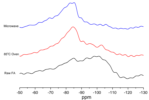
Fig. 3 29 Si NMR spectra of raw fly ash and AAFA under thermal oven curing and microwave curing
