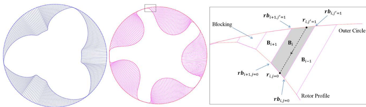
Figure 12 Background blocking for the main and gate rotors and projection function
