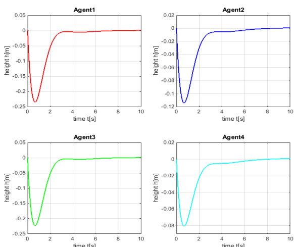
Fig. 6. Height response of the nonlinear LQR system controlled by the distributed controller in the presence of the impulse disturbance
