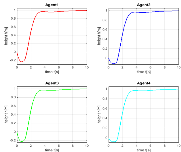
Fig. 5. Step height response of the linear LQR system controlled by the distributed controller in the presence of the impulse disturbance
