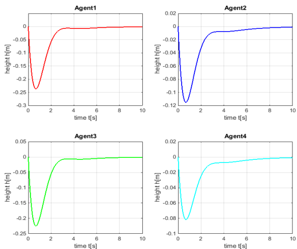
Fig. 3. Height response of the linear LQR system controlled by the distributed controller in the presence of the impulse disturbance
