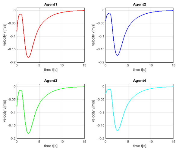
Fig. 4. Velocity response of the linear LQR system controlled by the distributed controller in the presence of the impulse disturbance
