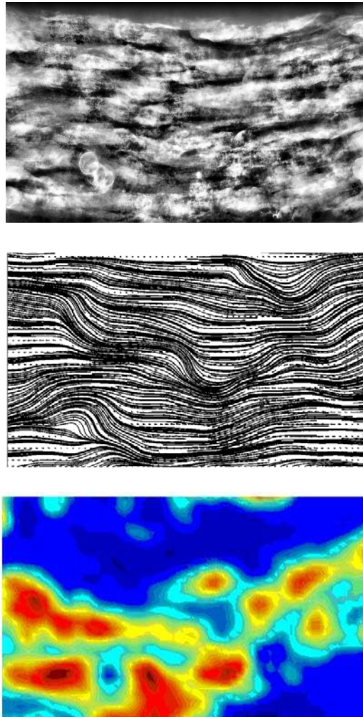
Fig. 8: Representation of the particle and fluid motion statistics: Top: Average of image sequence showing preferred paths of particles and events of particle contacts with the bottom wall. Center: streamlines of the liquid phase showing regions of large disturbances where the flow is forced to swirl around clusters or particles at rest. Bottom: regions of high fluctuation energy of fluid motion (color bar from \langle u^2 \rangle / U^2 = 0.1 in red to 0 in blue). Physical size of image area is 11.6 \times 7 \text{ mm}^2 .
