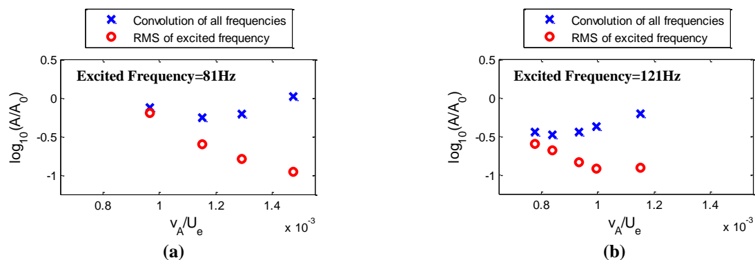
Figure 4. Effect of suction on single profiles located at a fixed position downstream ( x/C= 0.3408 ) of the suction insert panel: (a) shows U_e=8\text{m/s} ; (b) shows U_e=12\text{m/s} . A_0 represents the amplitude of the case with no suction and the perforations uncovered, and d_h=0.6\text{mm} for both cases.
