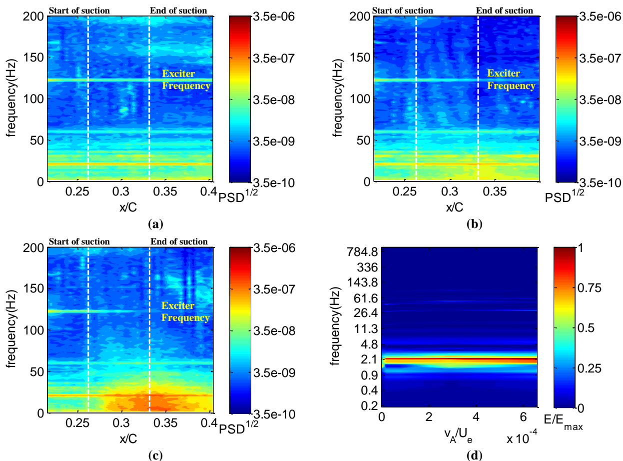
Figure 3. Power Spectral Density plots of Hot-wire and microphone sensors at z=0 mm, U_e=18 m/s, d_h=0.6 mm, and fk=121 Hz: (a) shows no suction with perforations covered, (b) shows v_A/U_e=0.0824E-3 , (c) shows v_A/U_e=0.2886E-3 of suction, (d) shows microphone energy for different suction rates.
