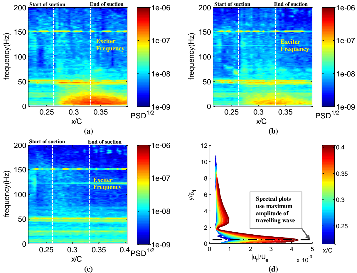
Figure 7. Three spectral plots for different cases and Travelling wave amplitude profile, all at U_e=14\text{m/s} , d_h=0.6\text{mm} , and f_k=121\text{Hz} : (a) shows with suction at v_A/U_e=0.8480E-3 , (b) shows no suction but perforations uncovered, (c) shows suction but with perforations covered, and (d) shows the point in the y -ordinate at which the spectral plots are shown.
