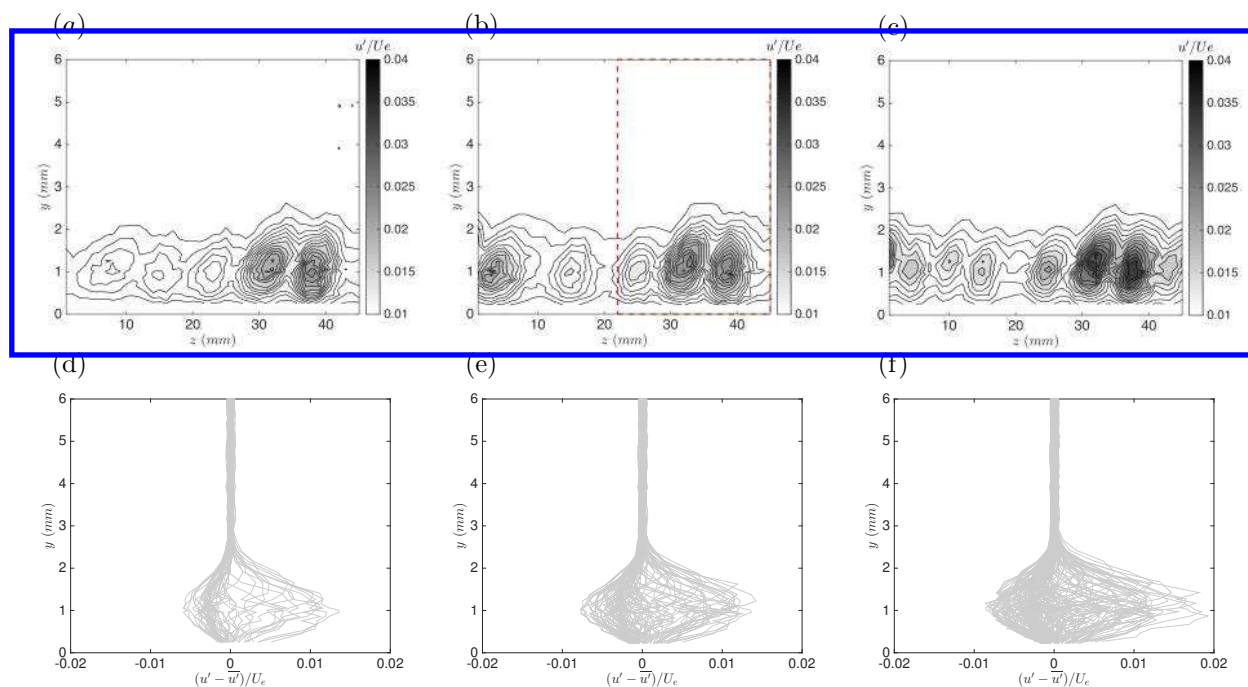
Figure 6. (top) Contour plots of non-dimensional fluctuating velocity profiles, u'/U_e , at x/c = 35\% for (a) Natural, (b) L11_H24_1R and (c) L11_H24_2R cases. (bottom) Respective 2D spanwise variation, (u' - \bar{u}')/U_e . The dashed red box in (b) is discussed in figure 8.
