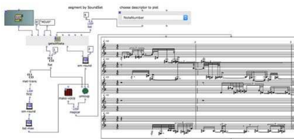
Figure 1. OPENMUSIC patch to transcribe an audio mosaic of a field recording.
