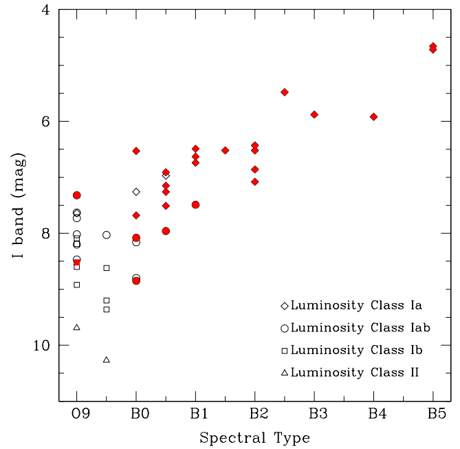
Fig. 5. Plot of I band magnitude versus spectral type for the late O - mid B stars within Wd1 (stars individually dereddened according to the prescription given in Negueruela et al. submitted). The photometric variables identified by Bonanos (2007) are indicated by the filled symbols.
