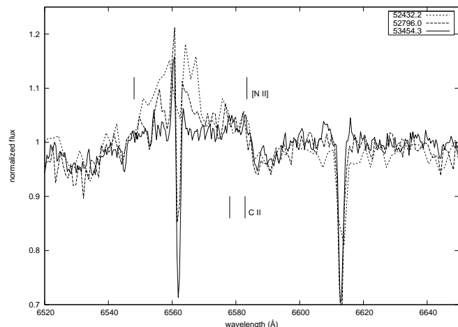
Fig. 13. LPV in H\alpha in W16a (A5 Ia + ) between 2002-5. Note the match between the strengths of the DIB in the 2003 & 2005 spectra implies that the change in strength of the narrow emission and absorption components is real. The location of C\text{II}\lambda\lambda 6578,82 and [N\text{II}]\lambda 6583 are also indicated.
