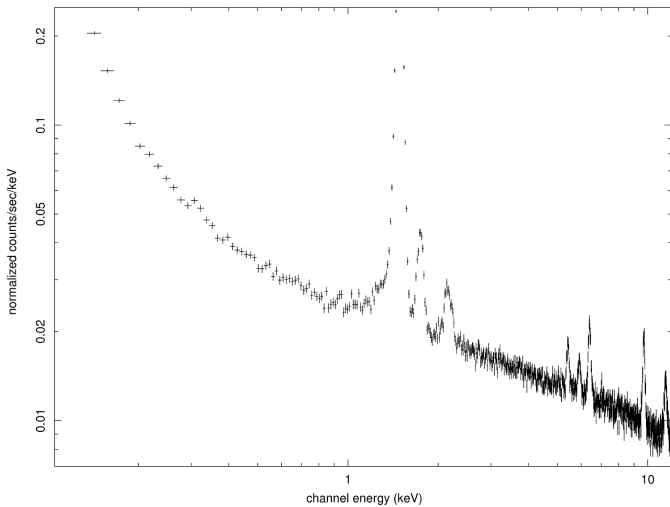
Fig. 1. The XMM-Newton MOS CCD instrument background, taken over the out-of-FOV regions of the CCD array through removing the circular FOV region and any anomalous areas - total area of approximately 11 \text{ cm}^2 .
