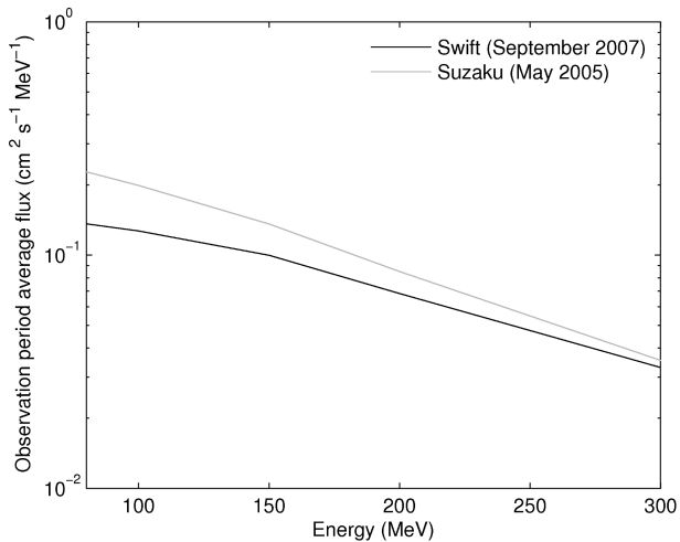
Fig. 6. The incident proton spectrum for the Suzaku mission in comparison to the Swift mission over the periods of in-orbit data collection (SPENVIS).
