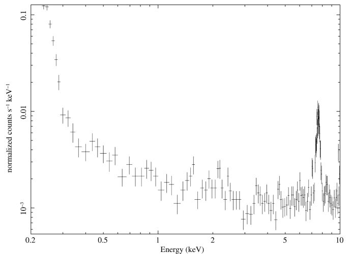
Fig. 2. The instrument background for the Swift MOS CCD (taken with the shutter closed over an area of 1.94 \text{ cm}^2 )
