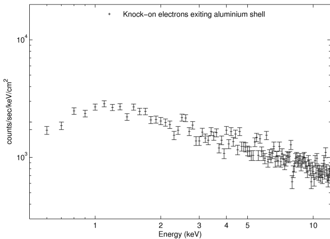
Fig. 9. The simulated spectrum of electrons emerging from the inner surface of the aluminium shell following bombardment with protons. These results were taken from the original simulation with the detector removed and all electrons emerging from the inner surface of the aluminium shell recorded.
