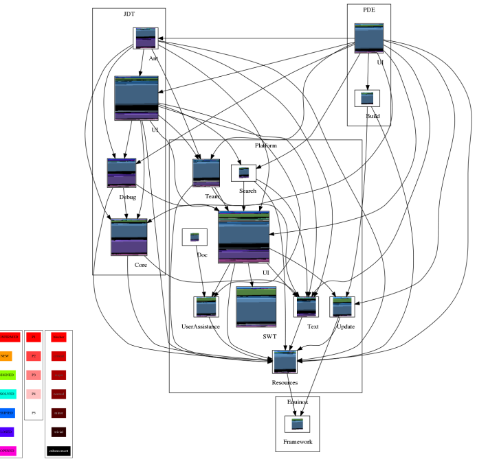
Figure 2. Annotating the Eclipse architecture graph with bugs reports
