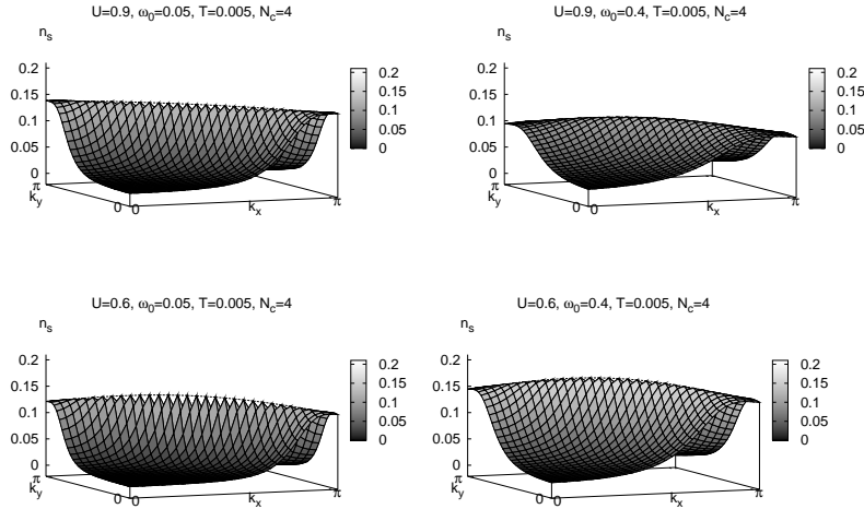
Figure 6. Variation of superconducting (anomalous) pairing density across the Brillouin zone. T = 0.005 and N_c = 4 . Changes in the order parameter are shown as coupling and phonon frequency are changed. As the phonon frequency is increased, the momentum dependence also increases, and the Fermi-surface is less well defined. For U = 0.9 , \omega_0 = 0.05 , the order parameter is almost flat along the Fermi-surface, indicating that DMFT is a good approximation for those parameters. For the largest coupling and phonon frequencies (at the edge of applicability for the current approximation), the Fermi-surface is practically destroyed.
