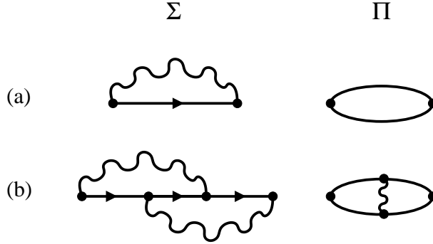
Figure 2. Diagrammatic representation of the approximation used in this paper. Series (a) represents the vertex-neglected theory which corresponds to the Migdal–Eliashberg approach. This is valid when there is a high probability that the last emitted phonon is the first to be reabsorbed, which is true if the phonon energy \omega_0 and electron-phonon coupling U are small compared to the Fermi energy. Series (b) represents additional diagrams for the vertex corrected theory. The inclusion of the lowest order vertex correction allows the order of absorption and emission of phonons to be swapped once. For moderate phonon frequency and electron-phonon coupling, these additions to the theory, in combination with non-local corrections are expected to improve the theory to sufficient accuracy. The phonon self energies are labeled with \Pi , and \Sigma denotes the electron self-energies. Lines represent the full electron Green’s function and wavy lines the full phonon Green’s function.
