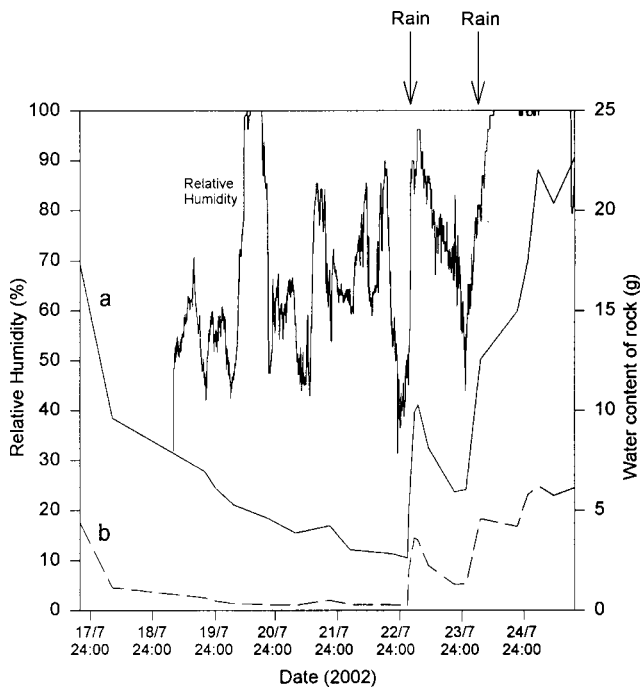
Fig. 4. Relative humidity (left-hand y-axis) measured during the rock moisture experiment from 21:00 on 17 July to 23:00 on 25 July. The right y-axis shows the mass gained (g) by two rocks, where the control mass was the dry mass. The dry masses were: (a) 207.2 g and (b) 68.9 g. Above the graph are the times at which rain occurred. In the first rain event 1 mm of water was deposited from 13:30 to 14:30 on 23 July. In the second rain event 4 mm of rain was deposited from 13:30 on 24 July to 0900 on 25 July, although light drizzle continued until the end of the experiment, hence the increasing rock mass.
