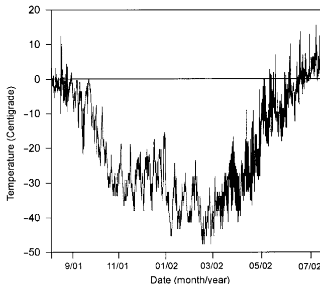
Fig. 3. Rock surface temperature from 16:00 on 14 August, 2001 to 10:00 on 10 July, 2002. The horizontal line in the graph denotes 0 °C.
