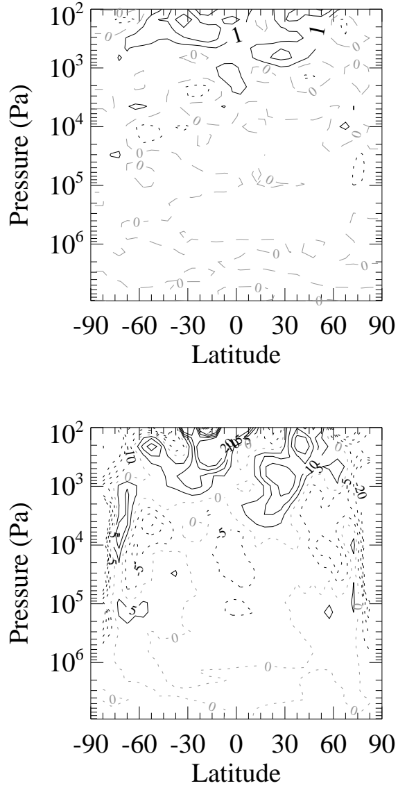
Figure 7: Individual terms in equation 8. Solid contours represent acceleration in each figure (regardless of sign), dotted contours represent deceleration , the grey dashed contour is the zero contour. (top) Net acceleration of the zonal mean angular momentum ( \overline{m}_t ), \Delta = 1 \text{ m}^2 \text{ s}^{-2} . (bottom) Acceleration of \overline{m} by the unresolved components in equation 8, calculated as the residual of the three preceding terms +F/\rho , \Delta = 5 \text{ m}^2 \text{ s}^{-2} . Figure 8 shows the TEM and Eliassen-Palm components.
