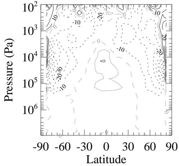
Figure 8: As figure 7. (top) Deceleration of \overline{m} by the mean circulation (\overline{\mathbf{u}}_* \cdot \nabla \overline{m}) , \Delta = 10 \text{ m}^2 \text{ s}^{-2} . (bottom) Acceleration of the \overline{m} by the resolved eddy components (-\nabla \cdot \mathbf{E}) , \Delta = 10 \text{ m}^2 \text{ s}^{-2} , the grey solid line is +5 \text{ m}^2 \text{ s}^{-2} .
