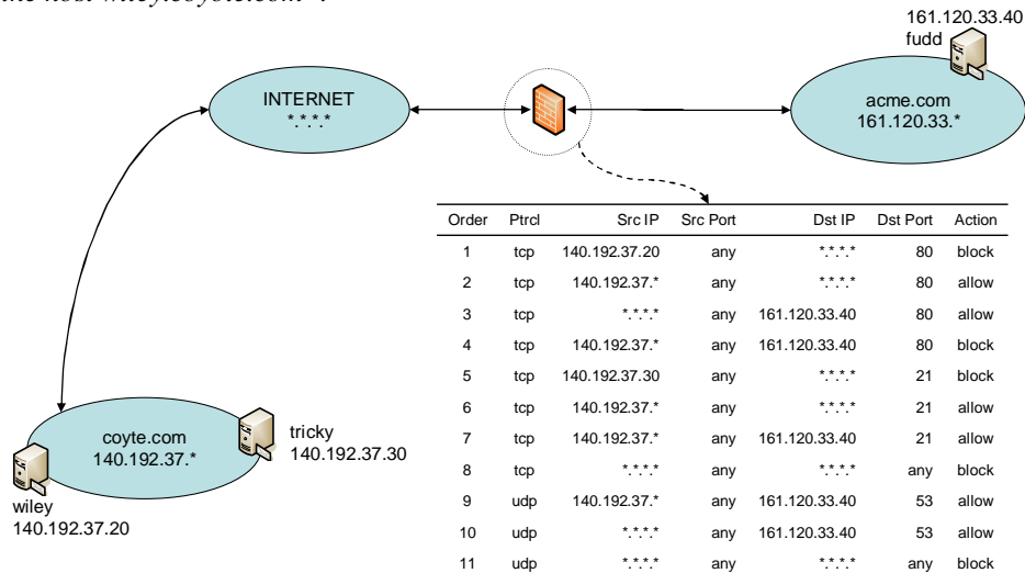
Fig. 1. Example network and associated firewall policy rules [1]
